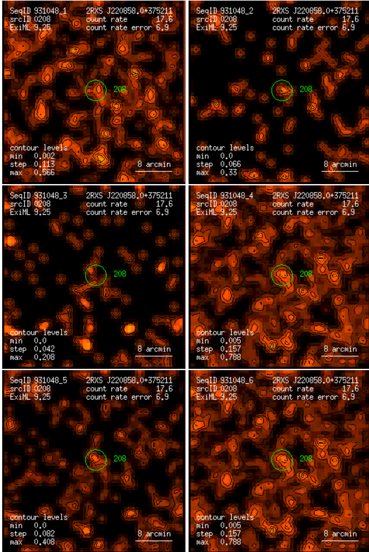
Figure 208: RASS 931048: detection 0208: band rate images, Gaussian filter: (1) PSPC channels 11 – 41, (2) 52 – 90, (3) 91 – 201, (4) 11 – 235, (5) 52 – 201, (6) 11 – 201. Broad band rates in counts/ks. Band rate contour levels in counts/ks/arcmin 2 .
