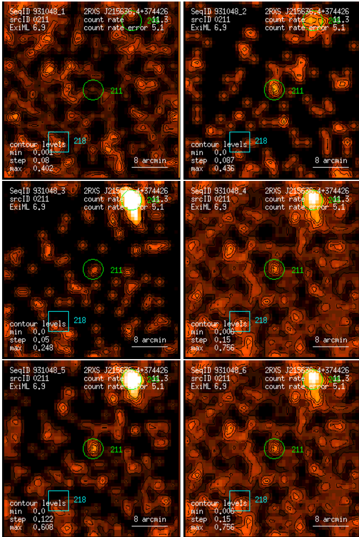
Figure 211: RASS 931048: detection 0211: band rate images, Gaussian filter: (1) PSPC channels 11 – 41, (2) 52 – 90, (3) 91 – 201, (4) 11 – 235, (5) 52 – 201, (6) 11 – 201. Broad band rates in counts/ks. Band rate contour levels in counts/ks/arcmin 2 .
