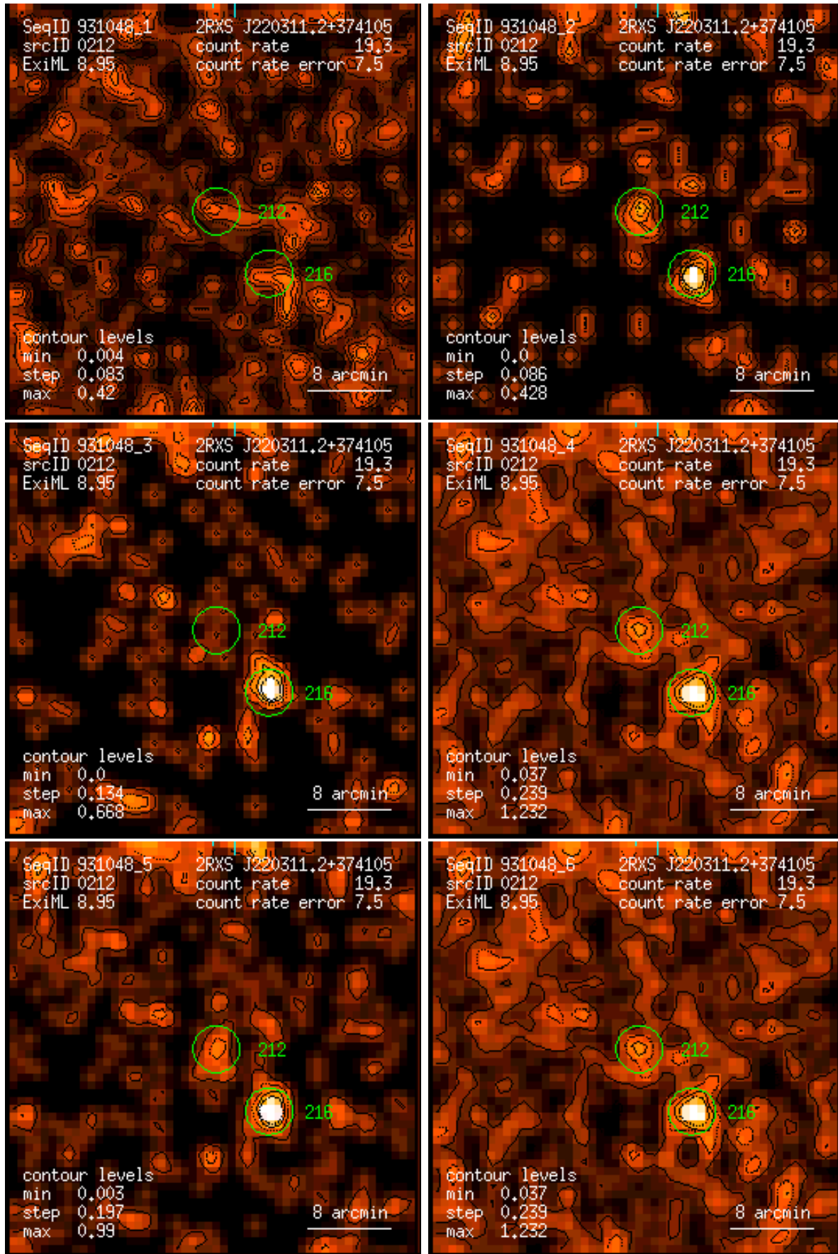
Figure 212: RASS 931048: detection 0212: band rate images, Gaussian filter: (1) PSPC channels 11 – 41, (2) 52 – 90, (3) 91 – 201, (4) 11 – 235, (5) 52 – 201, (6) 11 – 201. Broad band rates in counts/ks. Band rate contour levels in counts/ks/arcmin 2 .
