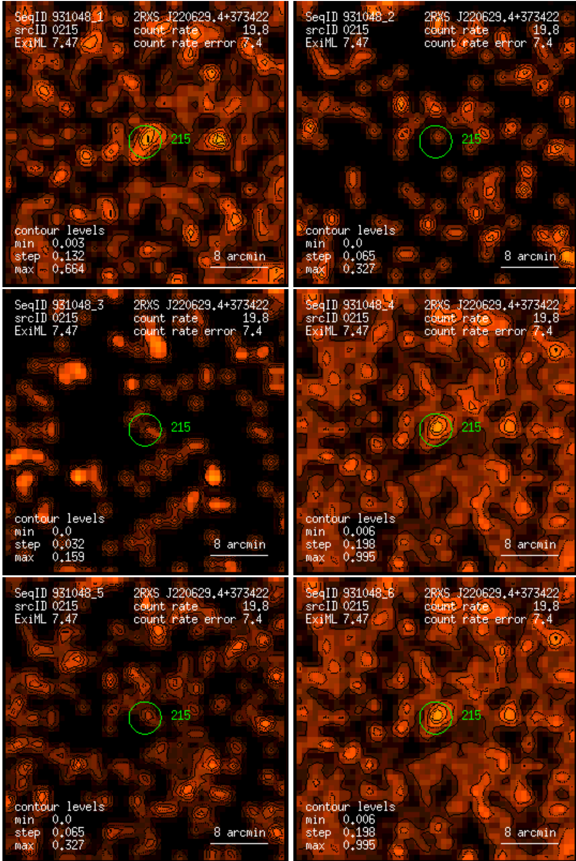
Figure 215: RASS 931048: detection 0215: band rate images, Gaussian filter: (1) PSPC channels 11 – 41, (2) 52 – 90, (3) 91 – 201, (4) 11 – 235, (5) 52 – 201, (6) 11 – 201. Broad band rates in counts/ks. Band rate contour levels in counts/ks/arcmin 2 .
