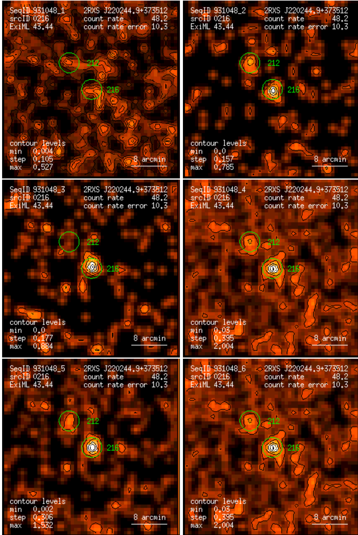
Figure 216: RASS 931048: detection 0216: band rate images, Gaussian filter: (1) PSPC channels 11 – 41, (2) 52 – 90, (3) 91 – 201, (4) 11 – 235, (5) 52 – 201, (6) 11 – 201. Broad band rates in counts/ks. Band rate contour levels in counts/ks/arcmin 2 .
