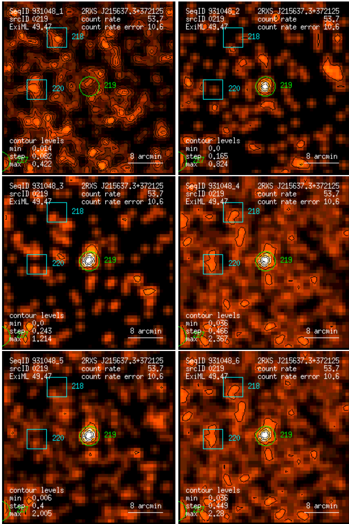
Figure 219: RASS 931048: detection 0219: band rate images, Gaussian filter: (1) PSPC channels 11 – 41, (2) 52 – 90, (3) 91 – 201, (4) 11 – 235, (5) 52 – 201, (6) 11 – 201. Broad band rates in counts/ks. Band rate contour levels in counts/ks/arcmin 2 .
