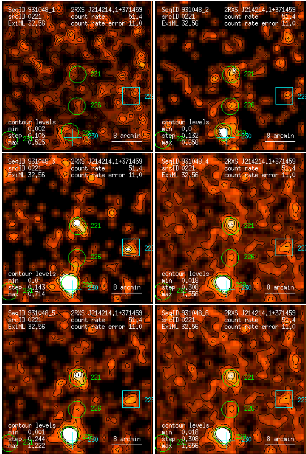
Figure 221: RASS 931048: detection 0221: band rate images, Gaussian filter: (1) PSPC channels 11 – 41, (2) 52 – 90, (3) 91 – 201, (4) 11 – 235, (5) 52 – 201, (6) 11 – 201. Broad band rates in counts/ks. Band rate contour levels in counts/ks/arcmin 2 .
