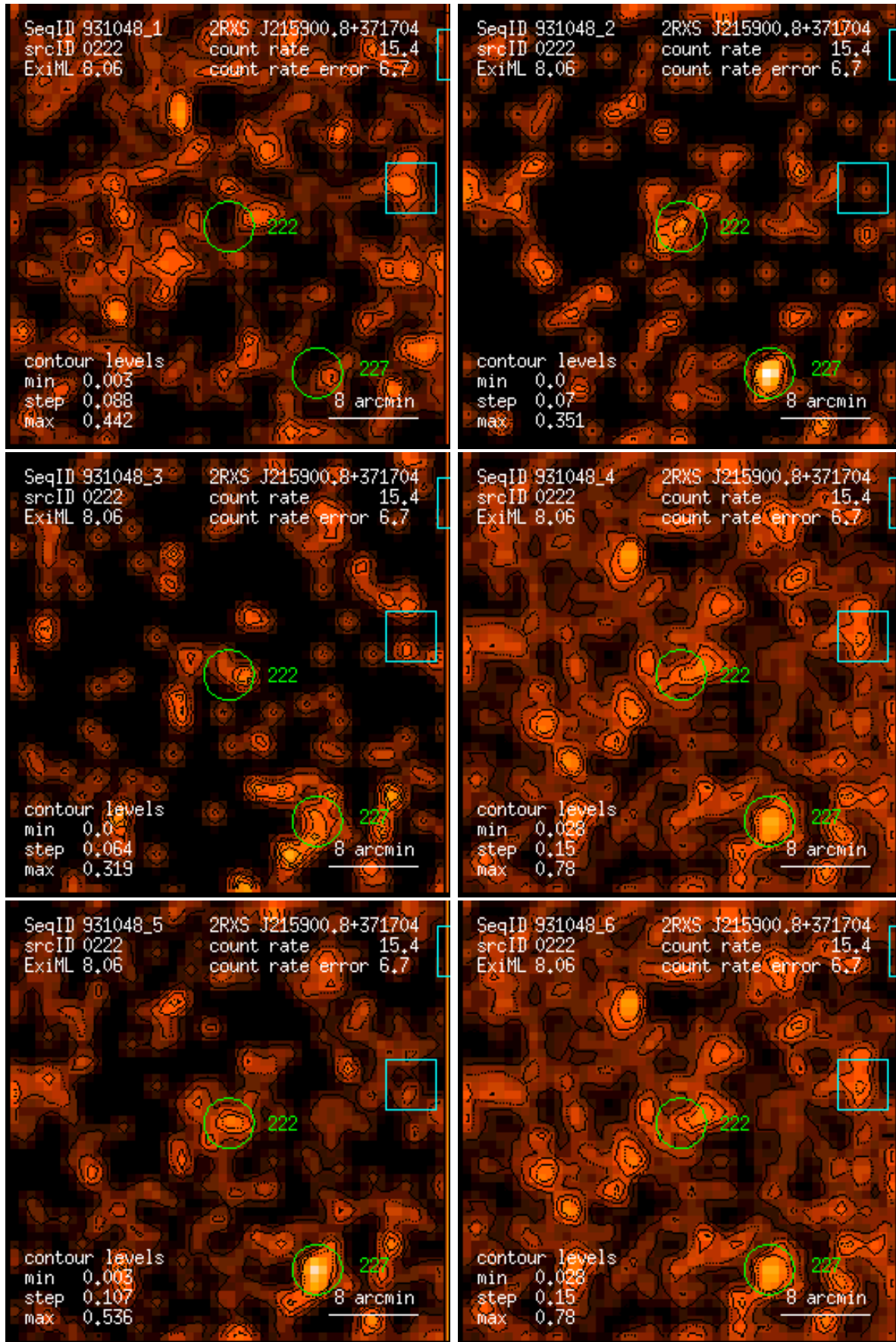
Figure 222: RASS 931048: detection 0222: band rate images, Gaussian filter: (1) PSPC channels 11 – 41, (2) 52 – 90, (3) 91 – 201, (4) 11 – 235, (5) 52 – 201, (6) 11 – 201. Broad band rates in counts/ks. Band rate contour levels in counts/ks/arcmin 2 .
