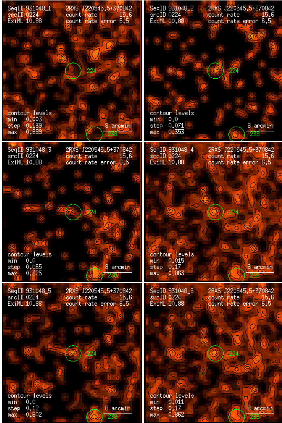
Figure 224: RASS 931048: detection 0224: band rate images, Gaussian filter: (1) PSPC channels 11 – 41, (2) 52 – 90, (3) 91 – 201, (4) 11 – 235, (5) 52 – 201, (6) 11 – 201. Broad band rates in counts/ks. Band rate contour levels in counts/ks/arcmin 2 .
