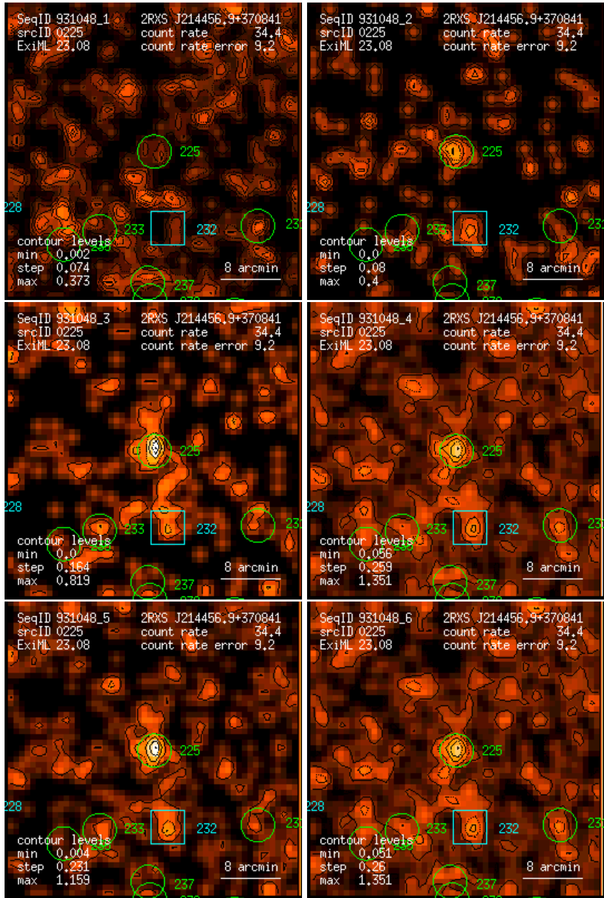
Figure 225: RASS 931048: detection 0225: band rate images, Gaussian filter: (1) PSPC channels 11 – 41, (2) 52 – 90, (3) 91 – 201, (4) 11 – 235, (5) 52 – 201, (6) 11 – 201. Broad band rates in counts/ks. Band rate contour levels in counts/ks/arcmin 2 .
