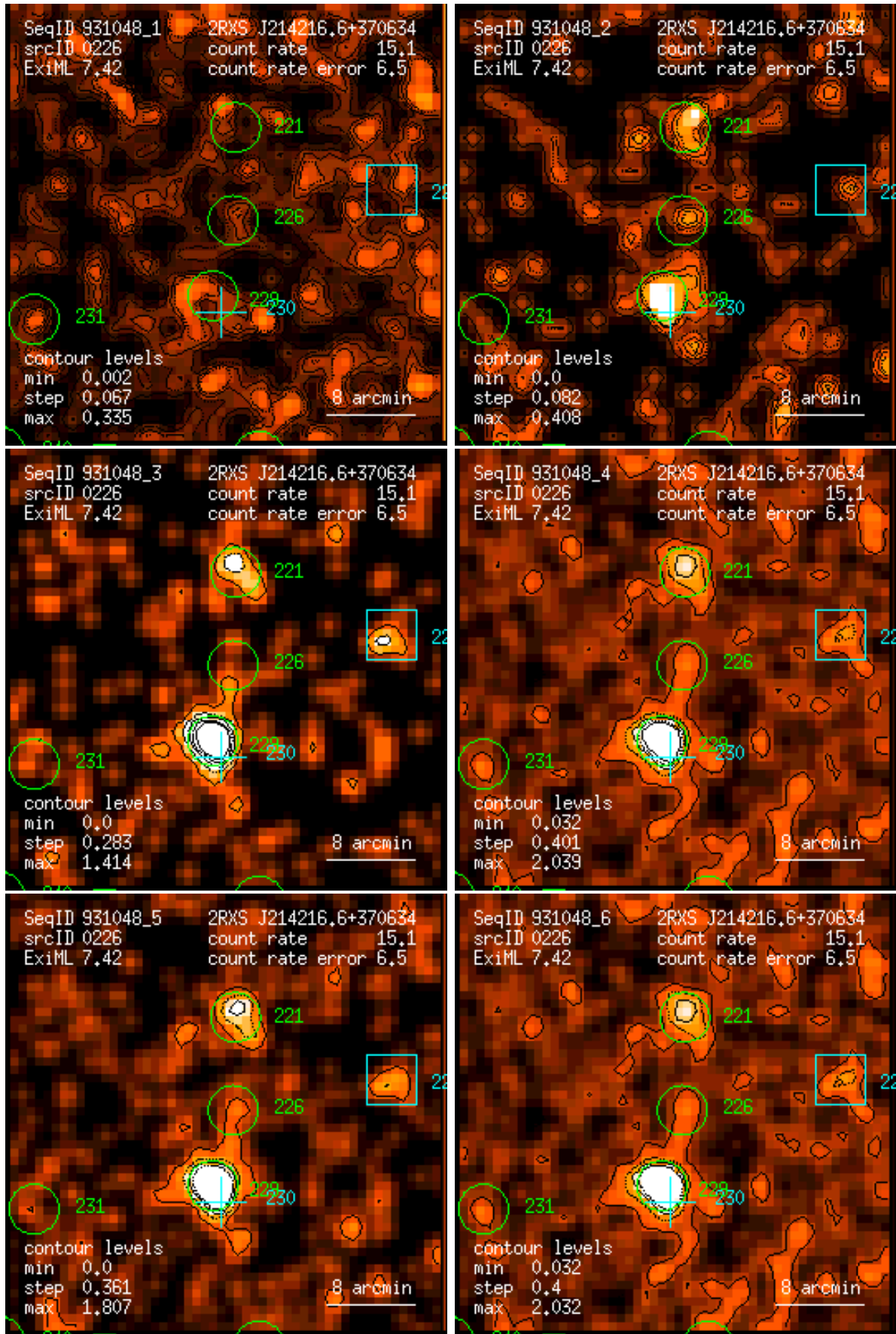
Figure 226: RASS 931048: detection 0226: band rate images, Gaussian filter: (1) PSPC channels 11 – 41, (2) 52 – 90, (3) 91 – 201, (4) 11 – 235, (5) 52 – 201, (6) 11 – 201. Broad band rates in counts/ks. Band rate contour levels in counts/ks/arcmin 2 .
