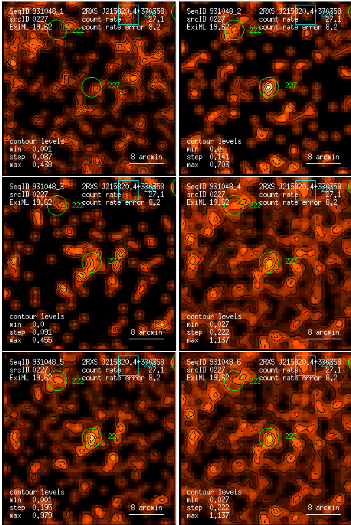
Figure 227: RASS 931048: detection 0227: band rate images, Gaussian filter: (1) PSPC channels 11 – 41, (2) 52 – 90, (3) 91 – 201, (4) 11 – 235, (5) 52 – 201, (6) 11 – 201. Broad band rates in counts/ks. Band rate contour levels in counts/ks/arcmin 2 .
