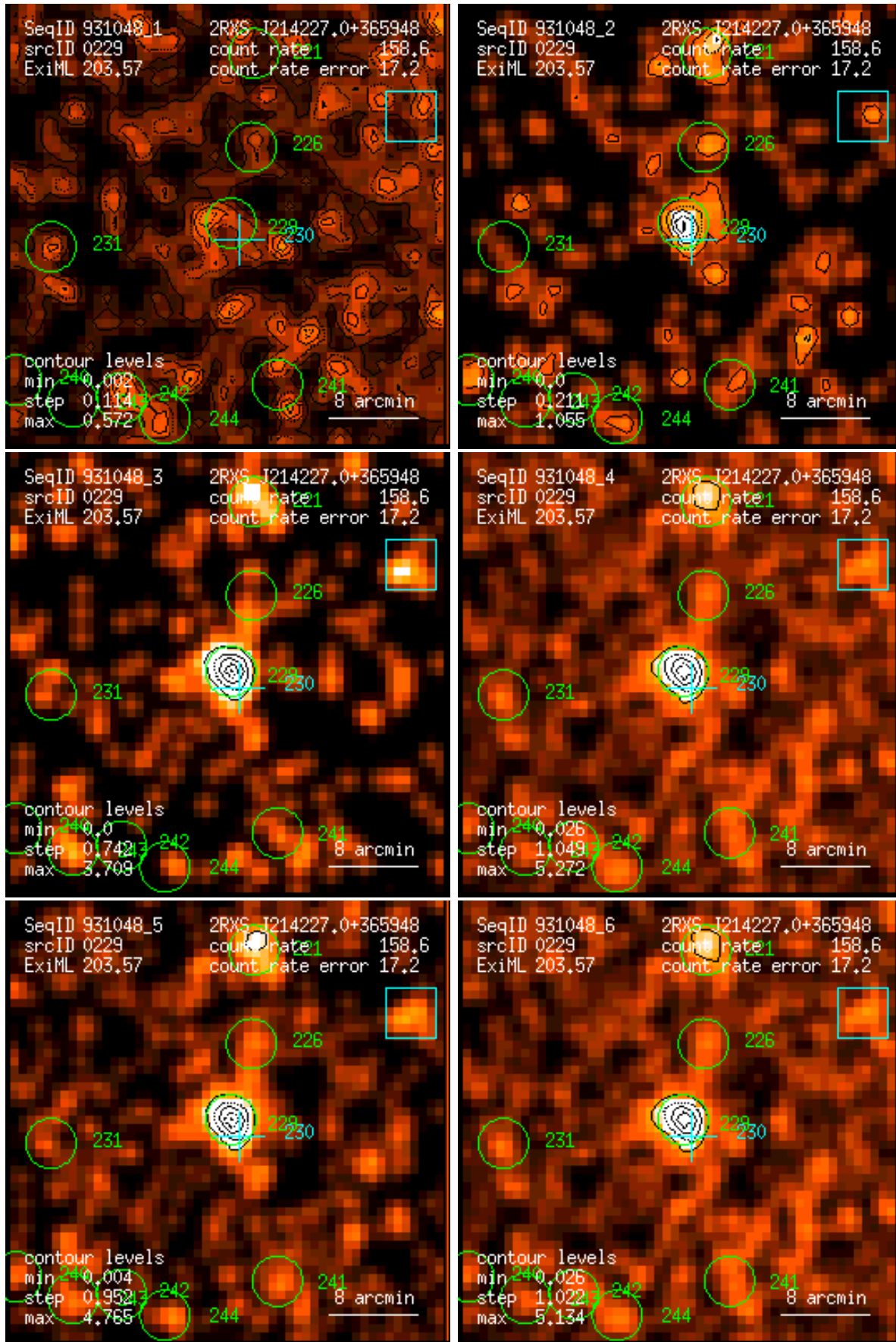
Figure 229: RASS 931048: detection 0229: band rate images, Gaussian filter: (1) PSPC channels 11 – 41, (2) 52 – 90, (3) 91 – 201, (4) 11 – 235, (5) 52 – 201, (6) 11 – 201. Broad band rates in counts/ks. Band rate contour levels in counts/ks/arcmin 2 .
