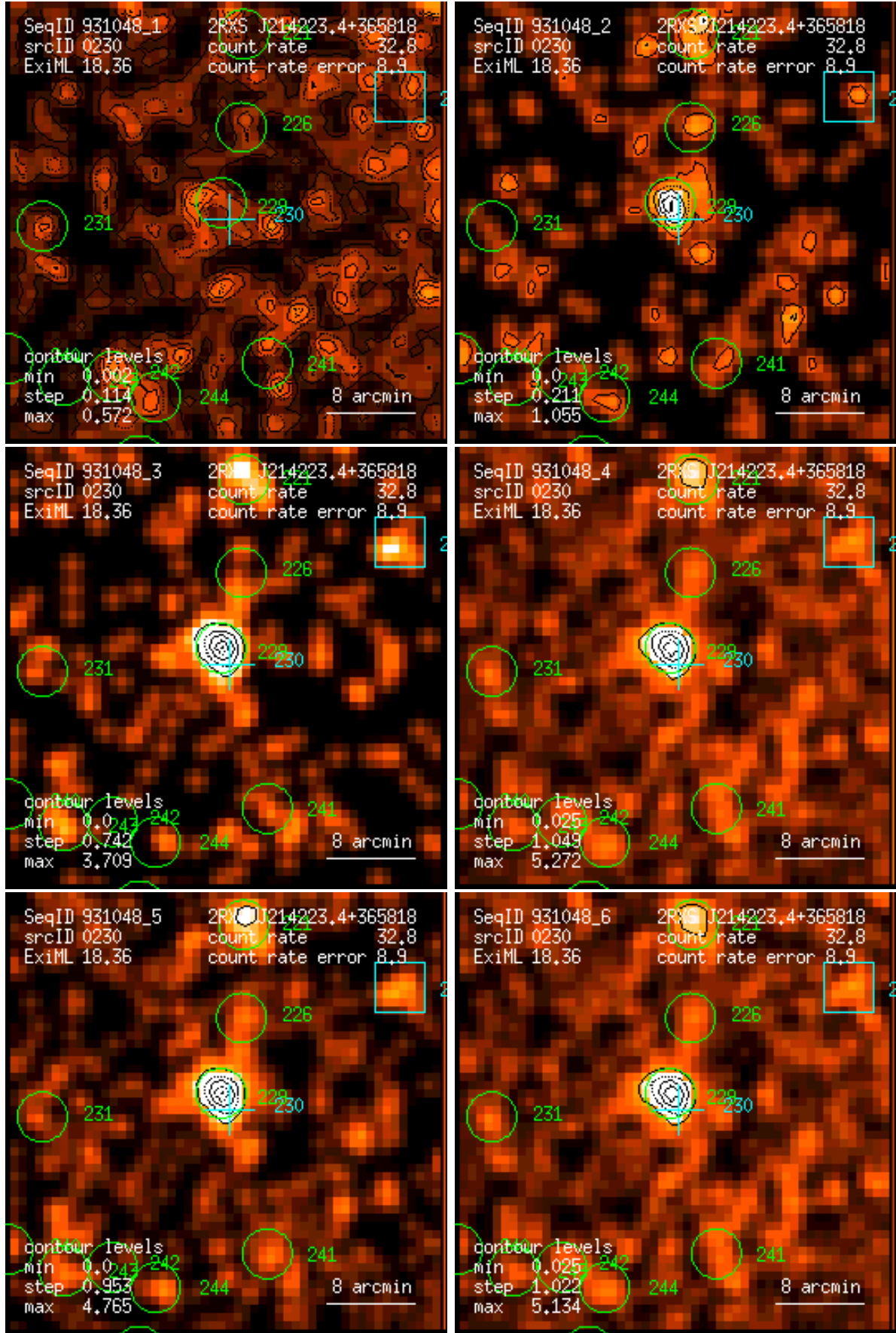
Figure 230: RASS 931048: detection 0230: band rate images, Gaussian filter: (1) PSPC channels 11 – 41, (2) 52 – 90, (3) 91 – 201, (4) 11 – 235, (5) 52 – 201, (6) 11 – 201. Broad band rates in counts/ks. Band rate contour levels in counts/ks/arcmin 2 .
