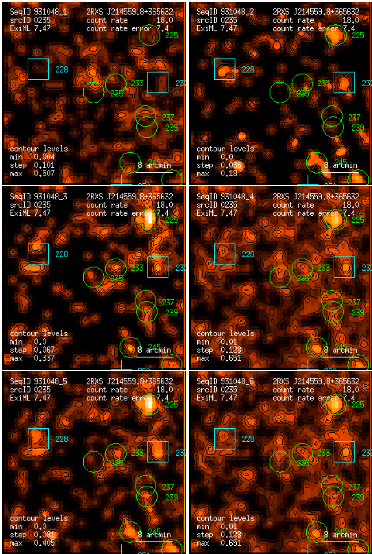
Figure 235: RASS 931048: detection 0235: band rate images, Gaussian filter: (1) PSPC channels 11 – 41, (2) 52 – 90, (3) 91 – 201, (4) 11 – 235, (5) 52 – 201, (6) 11 – 201. Broad band rates in counts/ks. Band rate contour levels in counts/ks/arcmin 2 .
