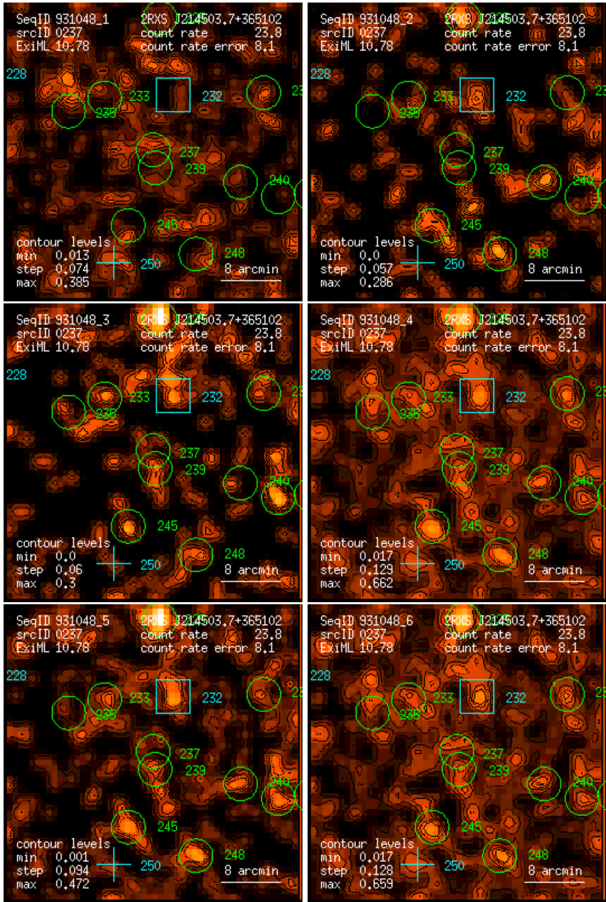
Figure 237: RASS 931048: detection 0237: band rate images, Gaussian filter: (1) PSPC channels 11 – 41, (2) 52 – 90, (3) 91 – 201, (4) 11 – 235, (5) 52 – 201, (6) 11 – 201. Broad band rates in counts/ks. Band rate contour levels in counts/ks/arcmin 2 .
