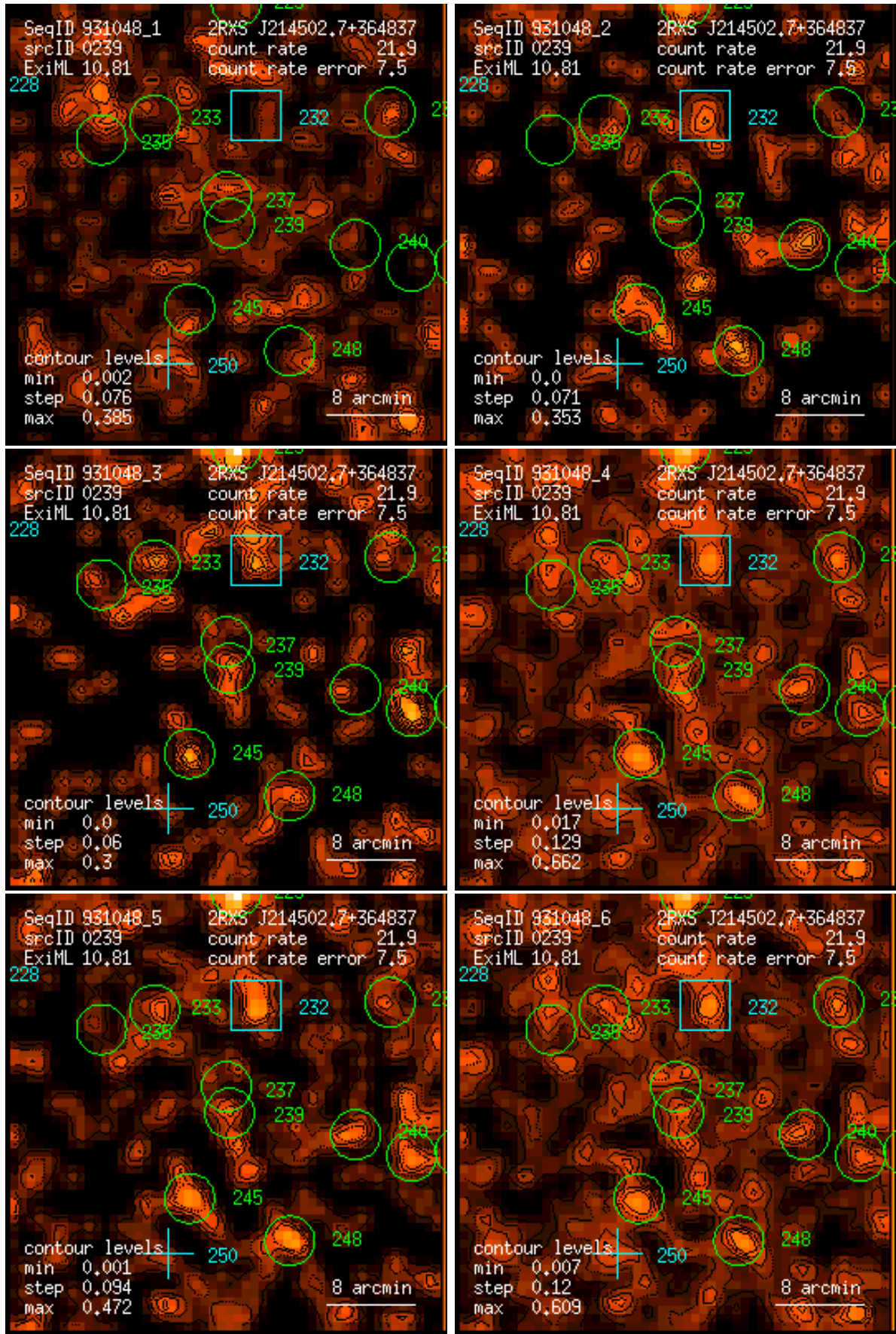
Figure 239: RASS 931048: detection 0239: band rate images, Gaussian filter: (1) PSPC channels 11 – 41, (2) 52 – 90, (3) 91 – 201, (4) 11 – 235, (5) 52 – 201, (6) 11 – 201. Broad band rates in counts/ks. Band rate contour levels in counts/ks/arcmin 2 .
