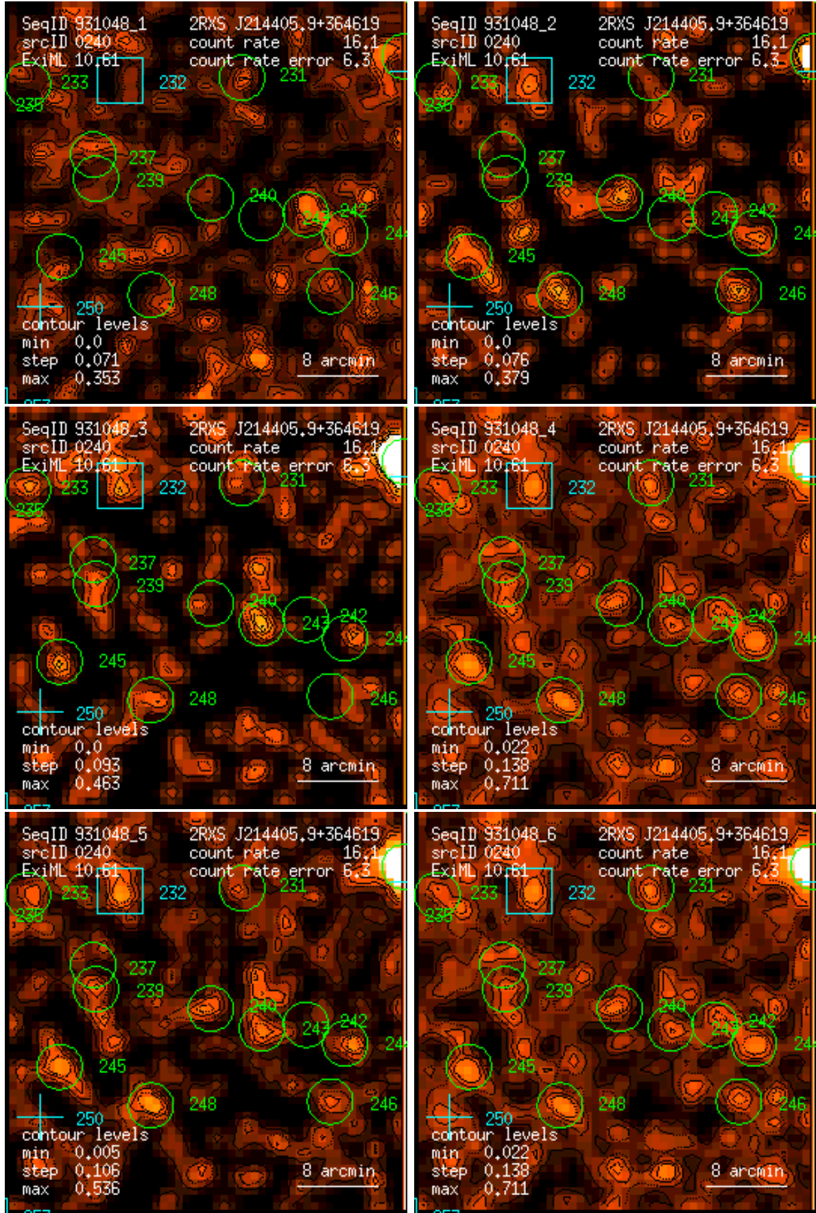
Figure 240: RASS 931048: detection 0240: band rate images, Gaussian filter: (1) PSPC channels 11 – 41, (2) 52 – 90, (3) 91 – 201, (4) 11 – 235, (5) 52 – 201, (6) 11 – 201. Broad band rates in counts/ks. Band rate contour levels in counts/ks/arcmin 2 .
