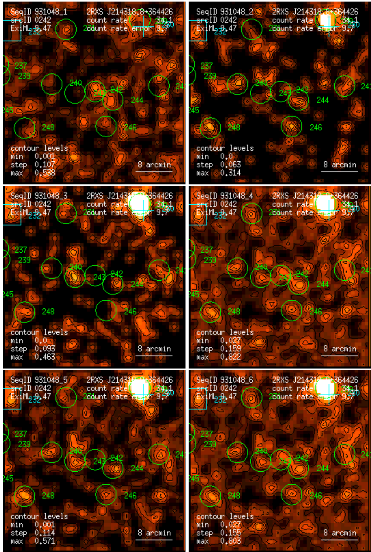
Figure 242: RASS 931048: detection 0242: band rate images, Gaussian filter: (1) PSPC channels 11 – 41, (2) 52 – 90, (3) 91 – 201, (4) 11 – 235, (5) 52 – 201, (6) 11 – 201. Broad band rates in counts/ks. Band rate contour levels in counts/ks/arcmin 2 .
