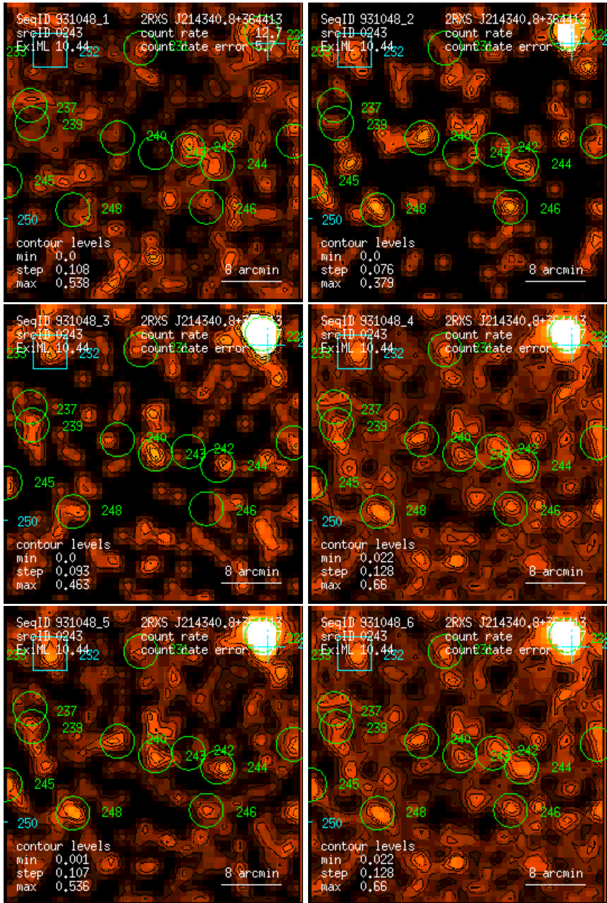
Figure 243: RASS 931048: detection 0243: band rate images, Gaussian filter: (1) PSPC channels 11 – 41, (2) 52 – 90, (3) 91 – 201, (4) 11 – 235, (5) 52 – 201, (6) 11 – 201. Broad band rates in counts/ks. Band rate contour levels in counts/ks/arcmin 2 .
