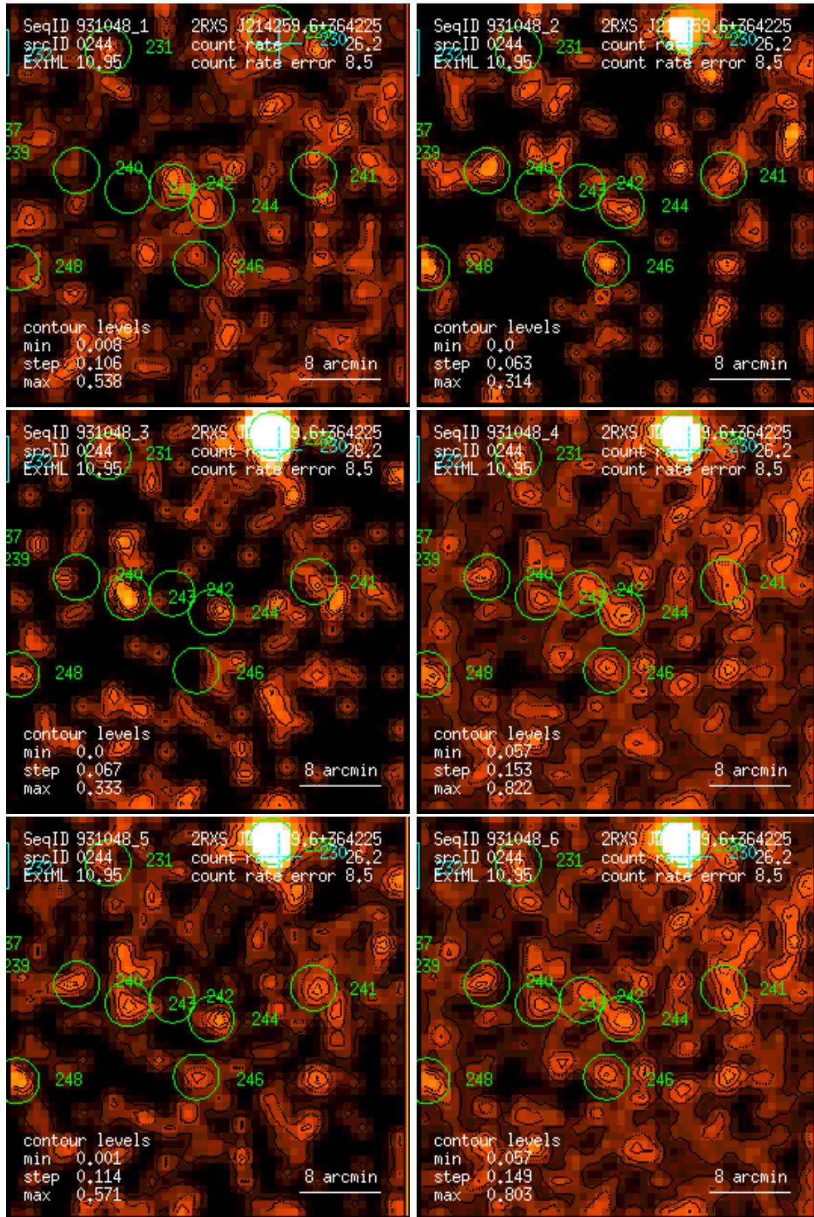
Figure 244: RASS 931048: detection 0244: band rate images, Gaussian filter: (1) PSPC channels 11 – 41, (2) 52 – 90, (3) 91 – 201, (4) 11 – 235, (5) 52 – 201, (6) 11 – 201. Broad band rates in counts/ks. Band rate contour levels in counts/ks/arcmin 2 .
