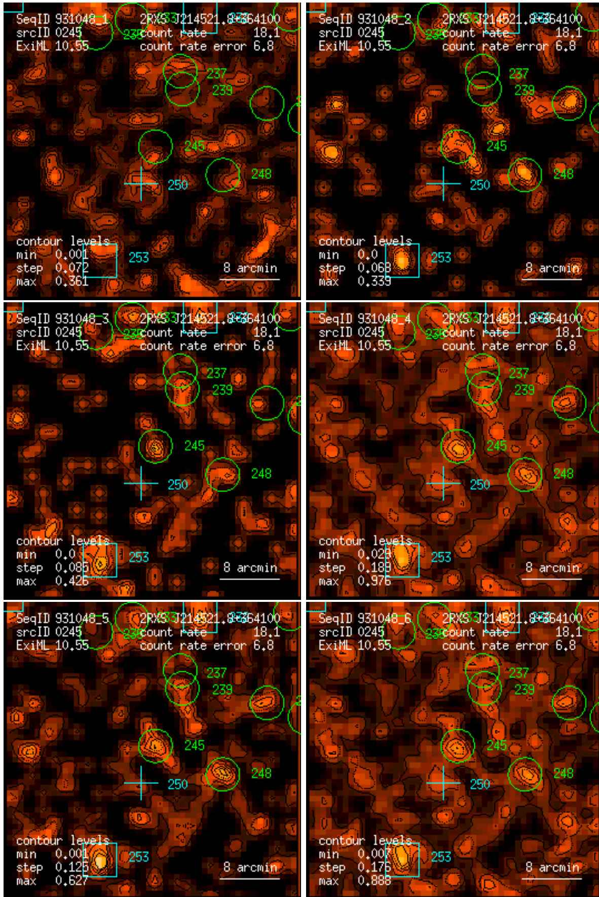
Figure 245: RASS 931048: detection 0245: band rate images, Gaussian filter: (1) PSPC channels 11 – 41, (2) 52 – 90, (3) 91 – 201, (4) 11 – 235, (5) 52 – 201, (6) 11 – 201. Broad band rates in counts/ks. Band rate contour levels in counts/ks/arcmin 2 .
