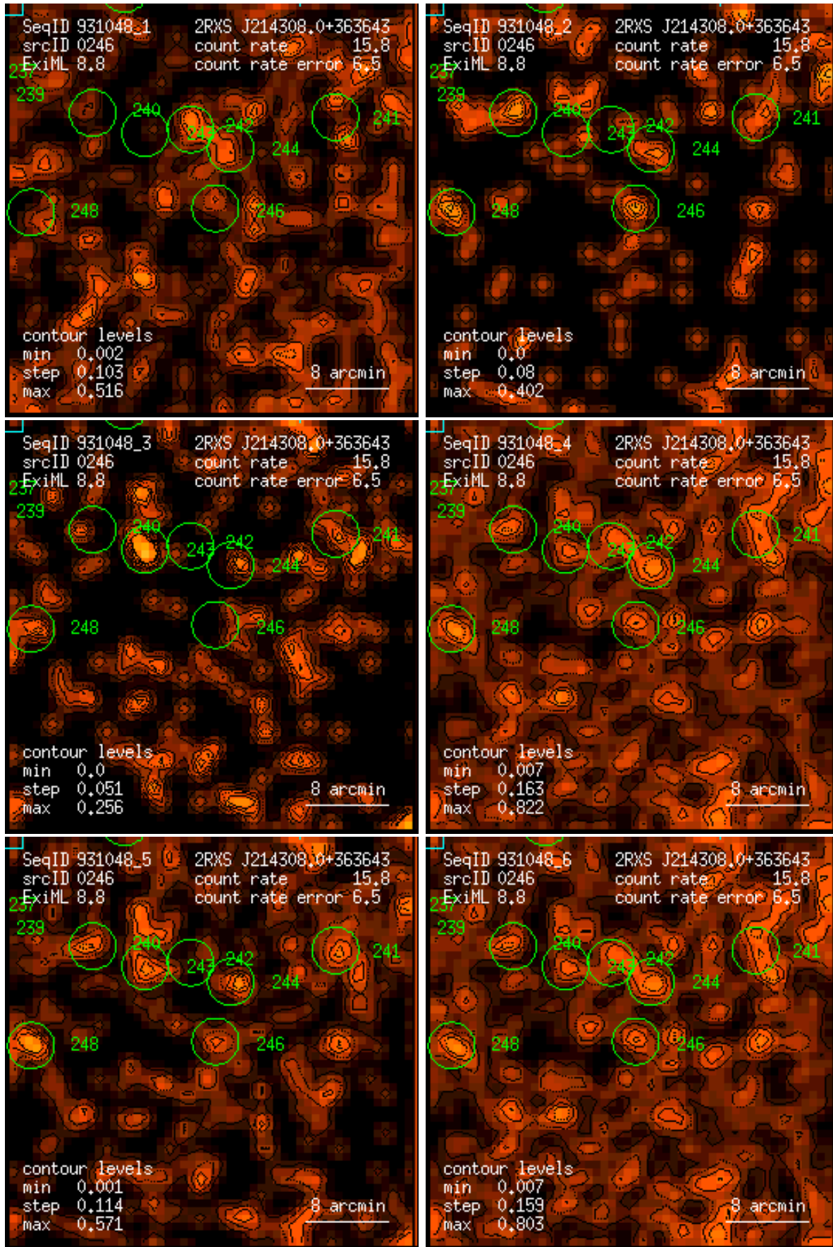
Figure 246: RASS 931048: detection 0246: band rate images, Gaussian filter: (1) PSPC channels 11 – 41, (2) 52 – 90, (3) 91 – 201, (4) 11 – 235, (5) 52 – 201, (6) 11 – 201. Broad band rates in counts/ks. Band rate contour levels in counts/ks/arcmin 2 .
