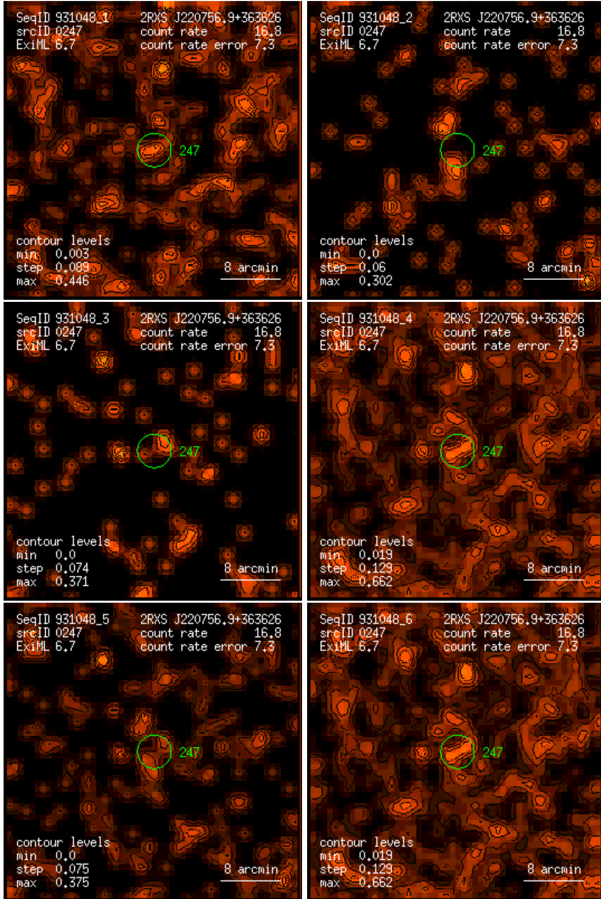
Figure 247: RASS 931048: detection 0247: band rate images, Gaussian filter: (1) PSPC channels 11 – 41, (2) 52 – 90, (3) 91 – 201, (4) 11 – 235, (5) 52 – 201, (6) 11 – 201. Broad band rates in counts/ks. Band rate contour levels in counts/ks/arcmin 2 .
