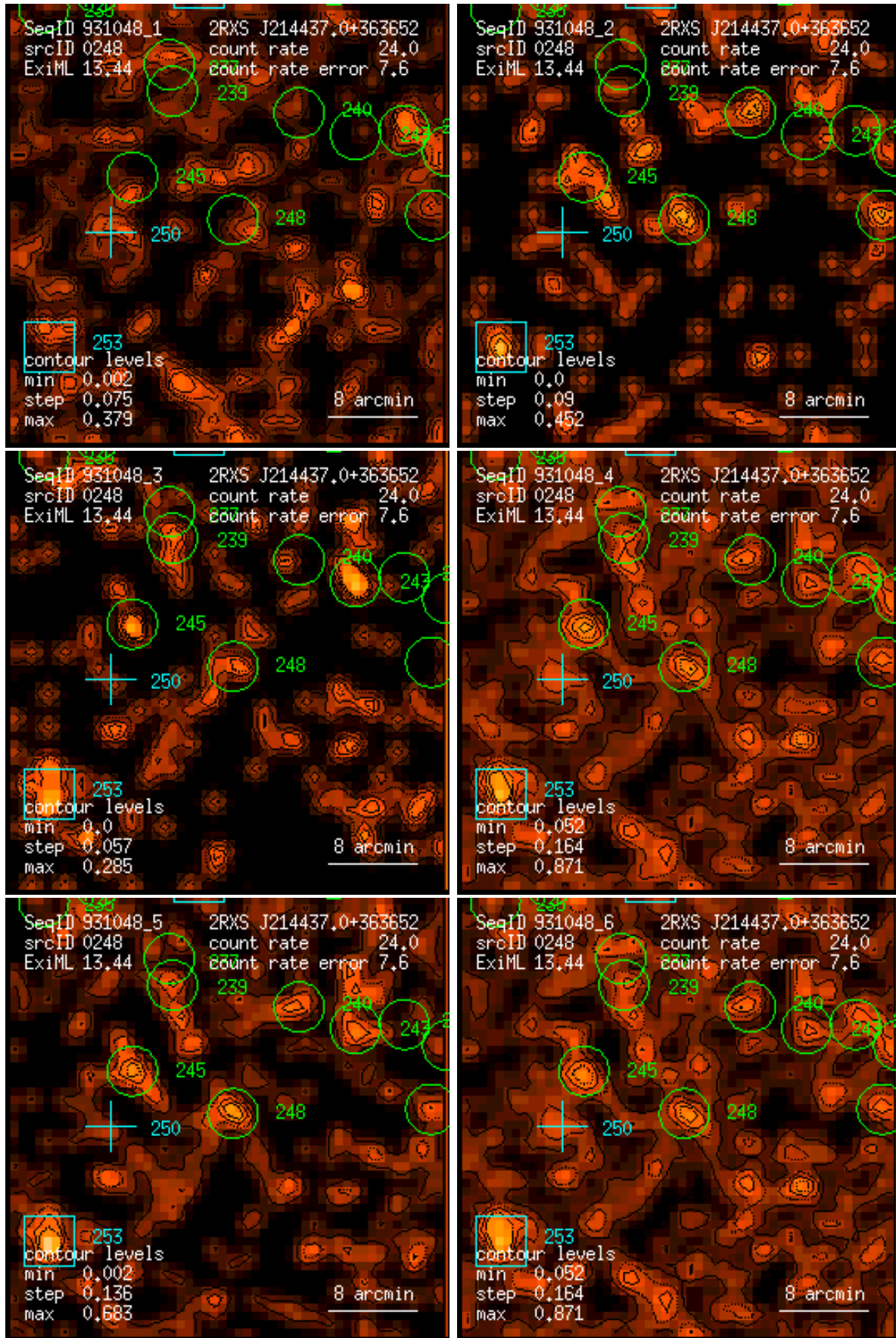
Figure 248: RASS 931048: detection 0248: band rate images, Gaussian filter: (1) PSPC channels 11 – 41, (2) 52 – 90, (3) 91 – 201, (4) 11 – 235, (5) 52 – 201, (6) 11 – 201. Broad band rates in counts/ks. Band rate contour levels in counts/ks/arcmin 2 .
