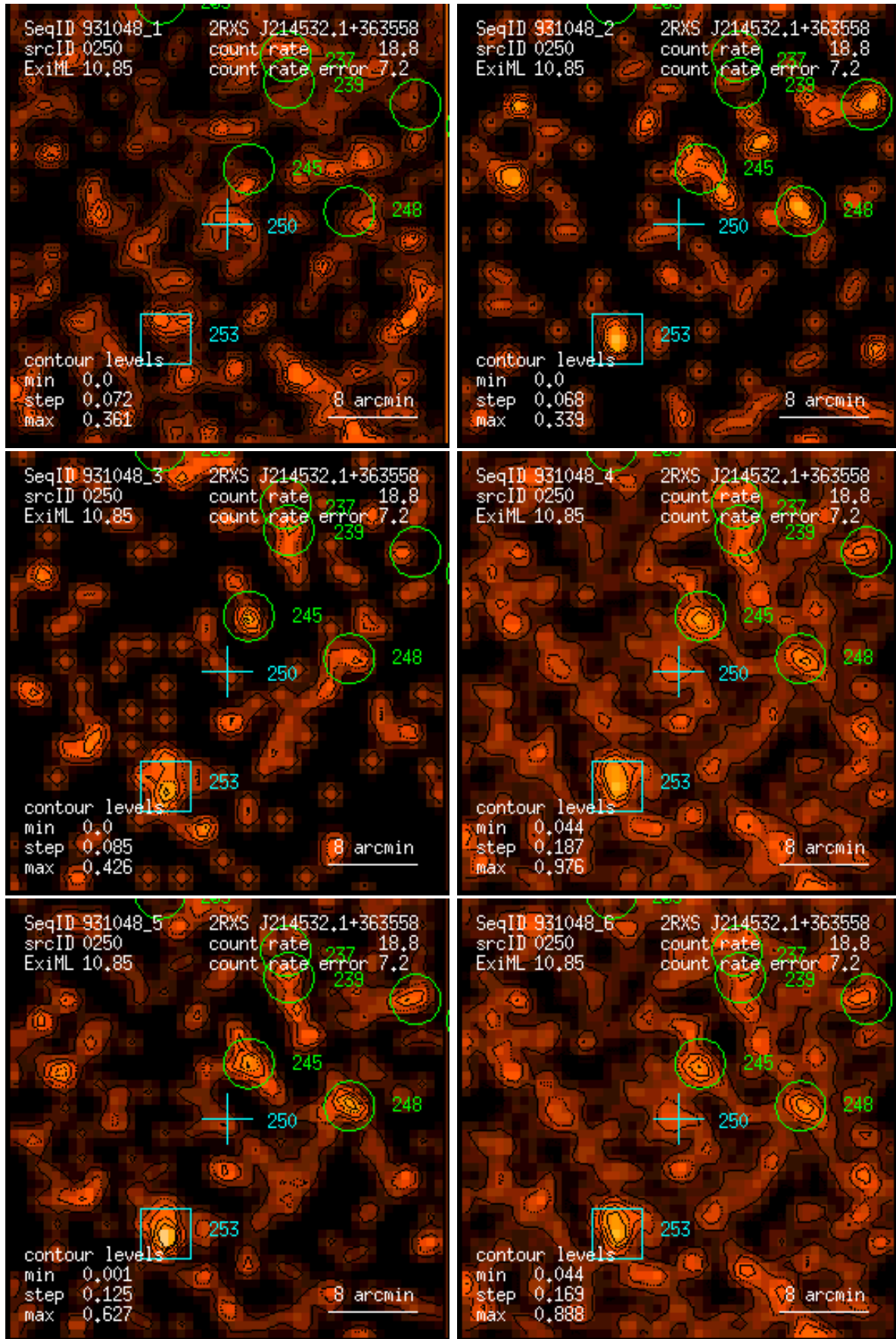
Figure 250: RASS 931048: detection 0250: band rate images, Gaussian filter: (1) PSPC channels 11 – 41, (2) 52 – 90, (3) 91 – 201, (4) 11 – 235, (5) 52 – 201, (6) 11 – 201. Broad band rates in counts/ks. Band rate contour levels in counts/ks/arcmin 2 .
