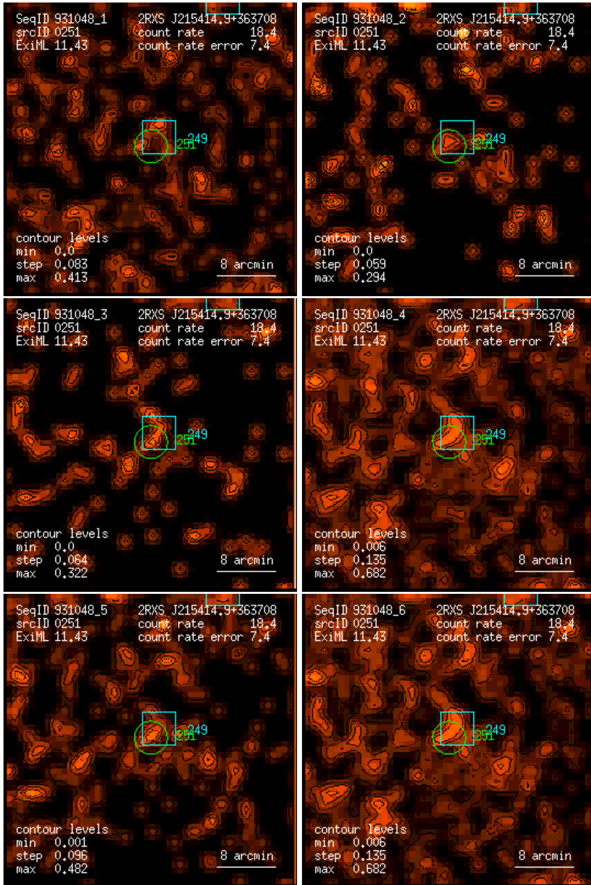
Figure 251: RASS 931048: detection 0251: band rate images, Gaussian filter: (1) PSPC channels 11 – 41, (2) 52 – 90, (3) 91 – 201, (4) 11 – 235, (5) 52 – 201, (6) 11 – 201. Broad band rates in counts/ks. Band rate contour levels in counts/ks/arcmin 2 .
