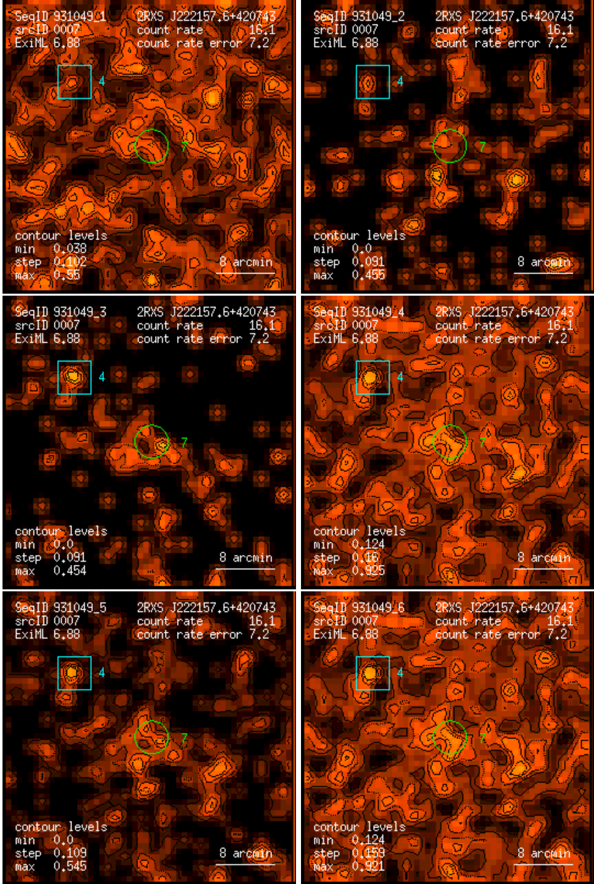
Figure 7: RASS 931049: detection 0007: band rate images, Gaussian filter: (1) PSPC channels 11 – 41, (2) 52 – 90, (3) 91 – 201, (4) 11 – 235, (5) 52 – 201, (6) 11 – 201. Broad band rates in counts/ks. Band rate contour levels in counts/ks/arcmin 2 .
