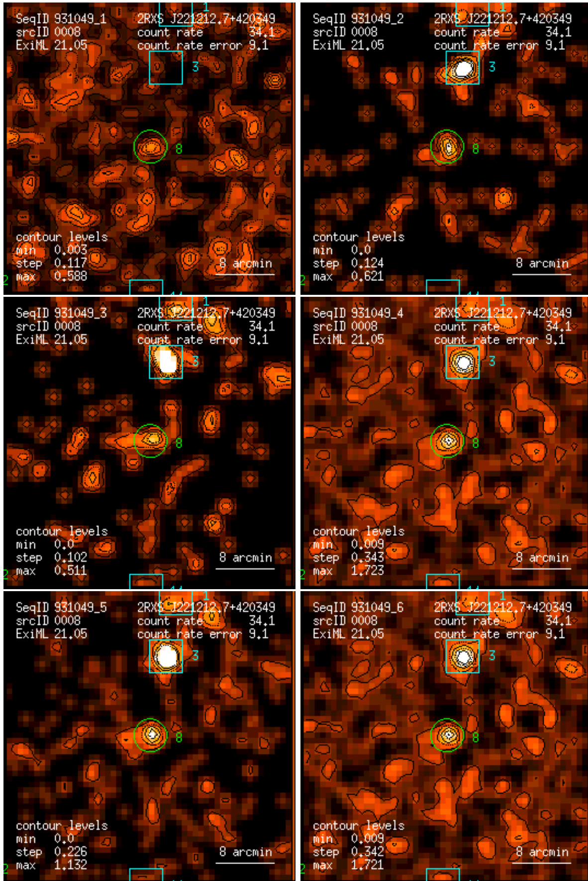
Figure 8: RASS 931049: detection 0008: band rate images, Gaussian filter: (1) PSPC channels 11 – 41, (2) 52 – 90, (3) 91 – 201, (4) 11 – 235, (5) 52 – 201, (6) 11 – 201. Broad band rates in counts/ks. Band rate contour levels in counts/ks/arcmin 2 .
