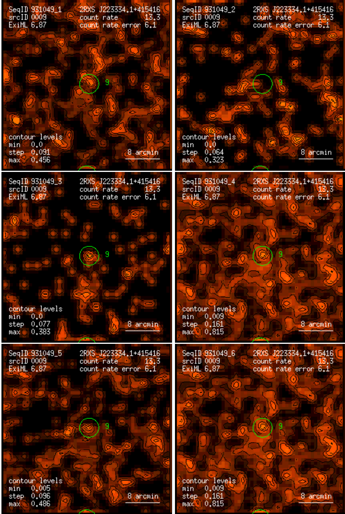
Figure 9: RASS 931049: detection 0009: band rate images, Gaussian filter: (1) PSPC channels 11 – 41, (2) 52 – 90, (3) 91 – 201, (4) 11 – 235, (5) 52 – 201, (6) 11 – 201. Broad band rates in counts/ks. Band rate contour levels in counts/ks/arcmin 2 .
