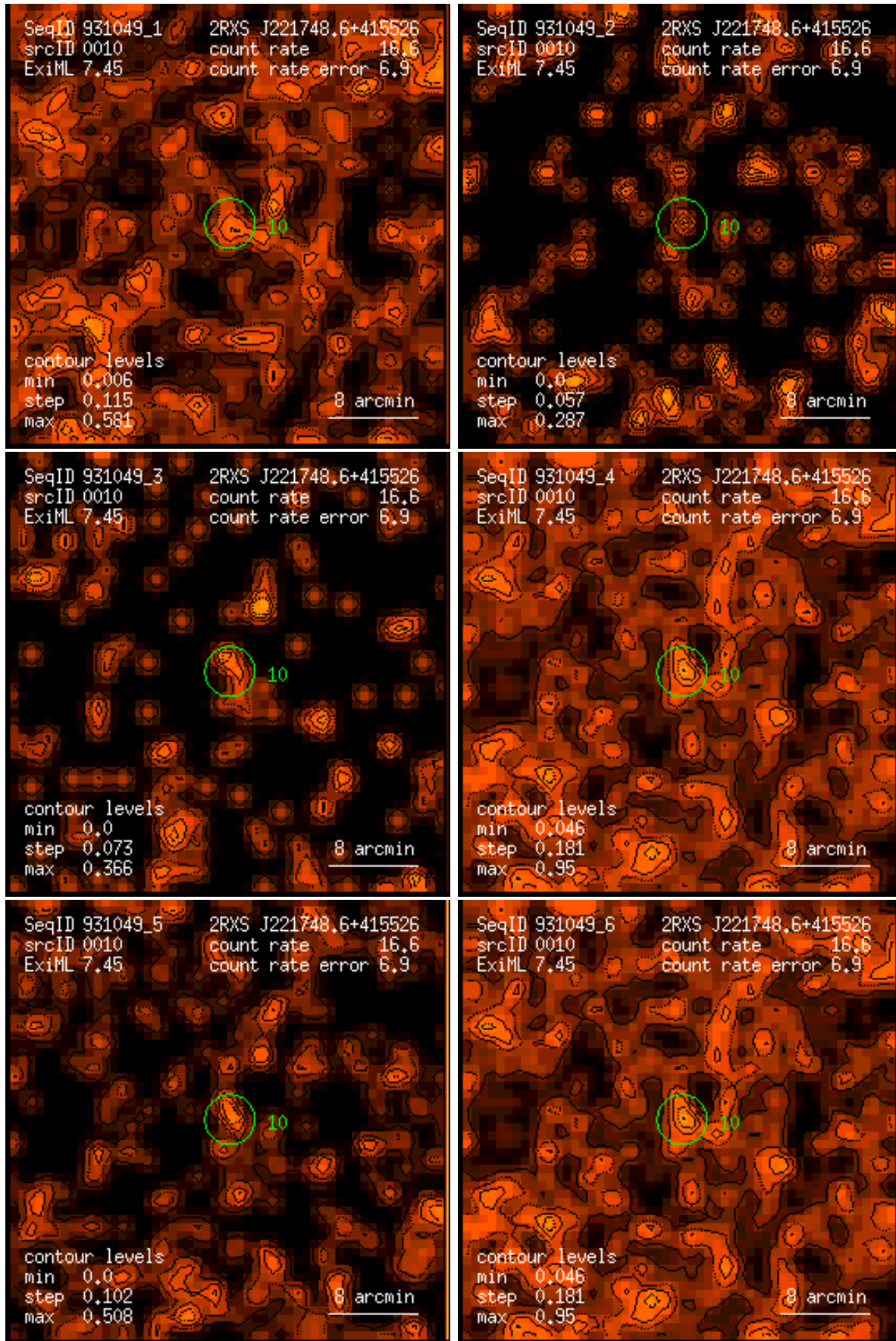
Figure 10: RASS 931049: detection 0010: band rate images, Gaussian filter: (1) PSPC channels 11 – 41, (2) 52 – 90, (3) 91 – 201, (4) 11 – 235, (5) 52 – 201, (6) 11 – 201. Broad band rates in counts/ks. Band rate contour levels in counts/ks/arcmin 2 .
