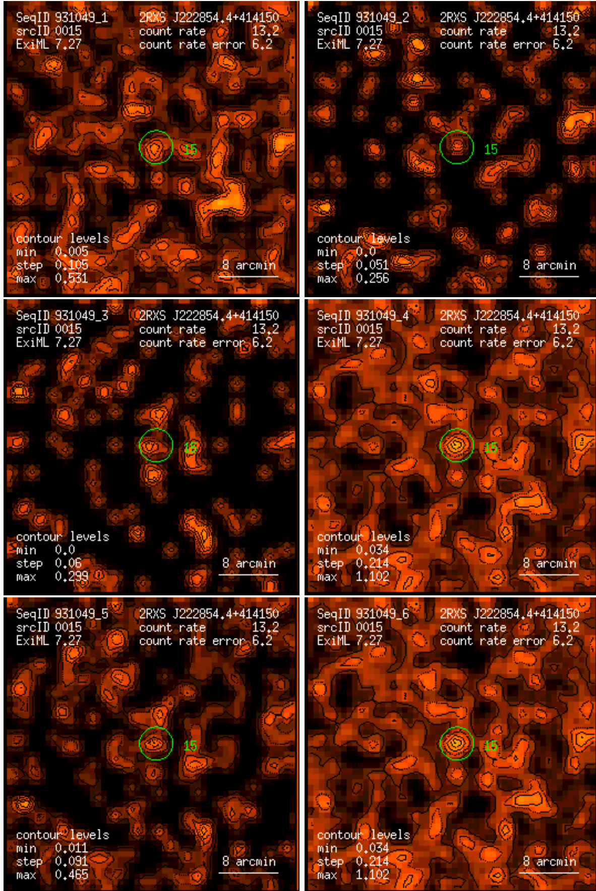
Figure 15: RASS 931049: detection 0015: band rate images, Gaussian filter: (1) PSPC channels 11 – 41, (2) 52 – 90, (3) 91 – 201, (4) 11 – 235, (5) 52 – 201, (6) 11 – 201. Broad band rates in counts/ks. Band rate contour levels in counts/ks/arcmin 2 .
