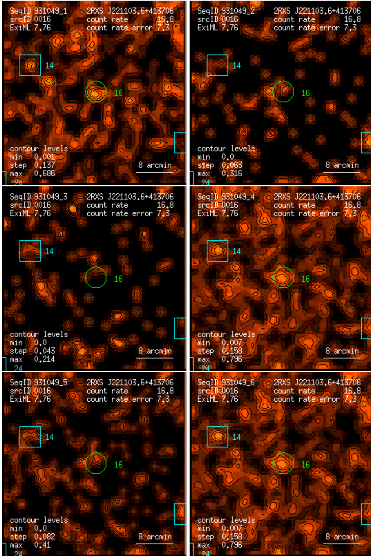
Figure 16: RASS 931049: detection 0016: band rate images, Gaussian filter: (1) PSPC channels 11 – 41, (2) 52 – 90, (3) 91 – 201, (4) 11 – 235, (5) 52 – 201, (6) 11 – 201. Broad band rates in counts/ks. Band rate contour levels in counts/ks/arcmin 2 .
