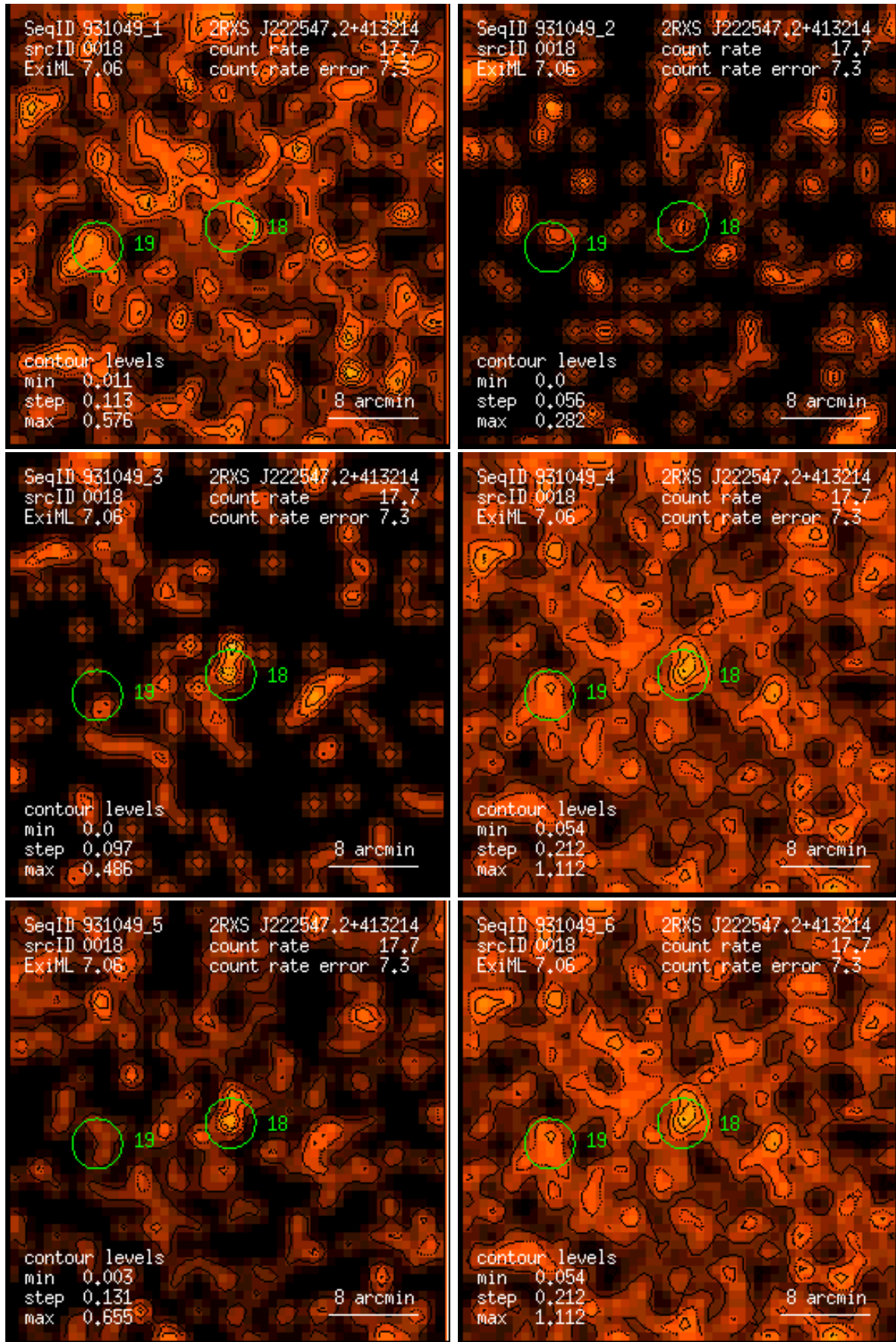
Figure 18: RASS 931049: detection 0018: band rate images, Gaussian filter: (1) PSPP channels 11 – 41, (2) 52 – 90, (3) 91 – 201, (4) 11 – 235, (5) 52 – 201, (6) 11 – 201. Broad band rates in counts/ks. Band rate contour levels in counts/ks/arcmin 2 .
