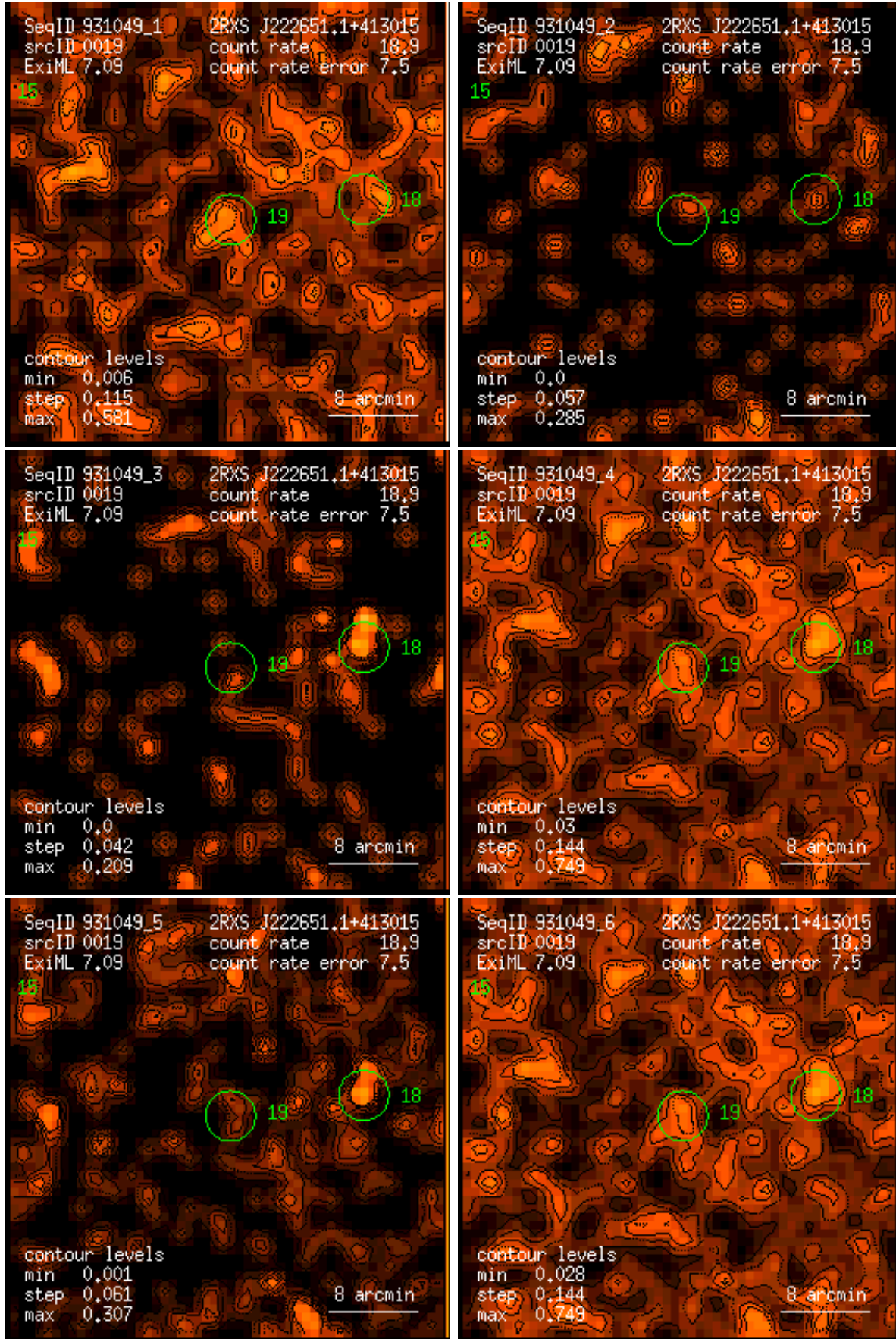
Figure 19: RASS 931049: detection 0019: band rate images, Gaussian filter: (1) PSPC channels 11 – 41, (2) 52 – 90, (3) 91 – 201, (4) 11 – 235, (5) 52 – 201, (6) 11 – 201. Broad band rates in counts/ks. Band rate contour levels in counts/ks/arcmin 2 .
