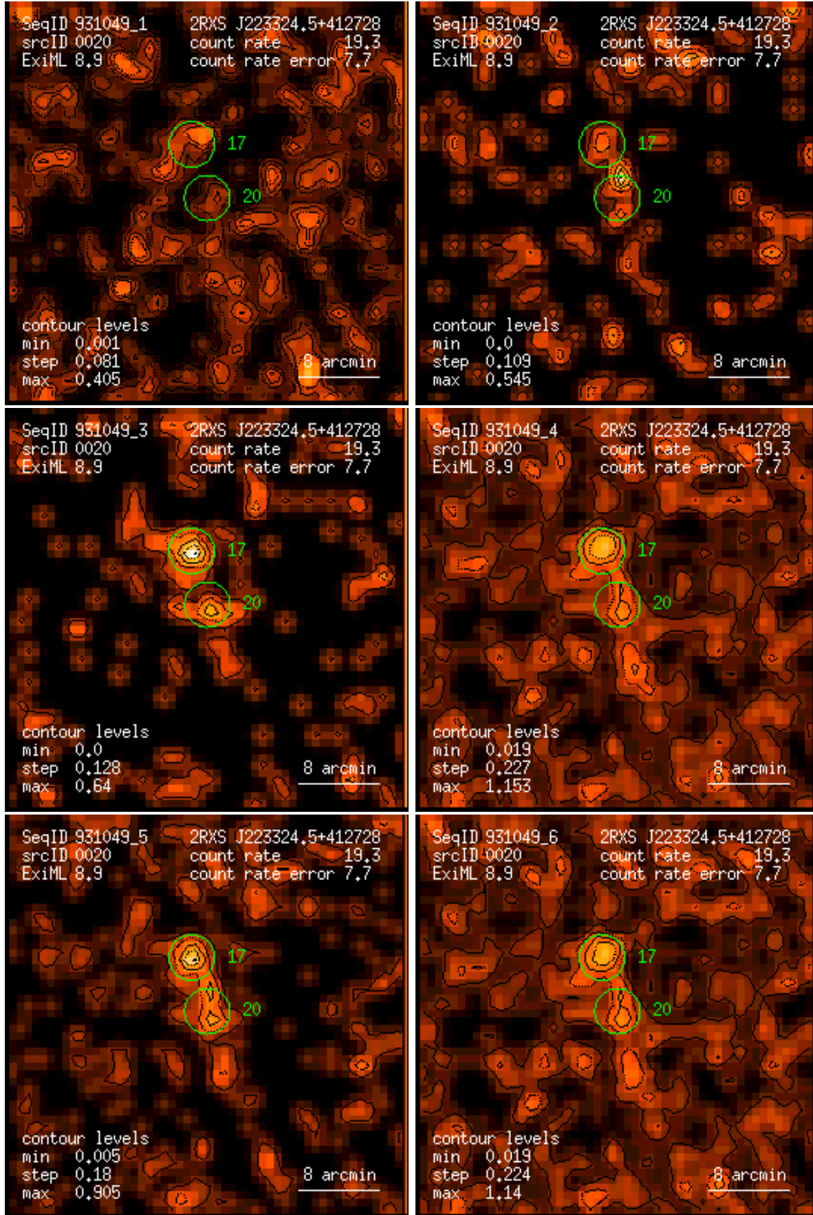
Figure 20: RASS 931049: detection 0020: band rate images, Gaussian filter: (1) PSPC channels 11 – 41, (2) 52 – 90, (3) 91 – 201, (4) 11 – 235, (5) 52 – 201, (6) 11 – 201. Broad band rates in counts/ks. Band rate contour levels in counts/ks/arcmin 2 .
