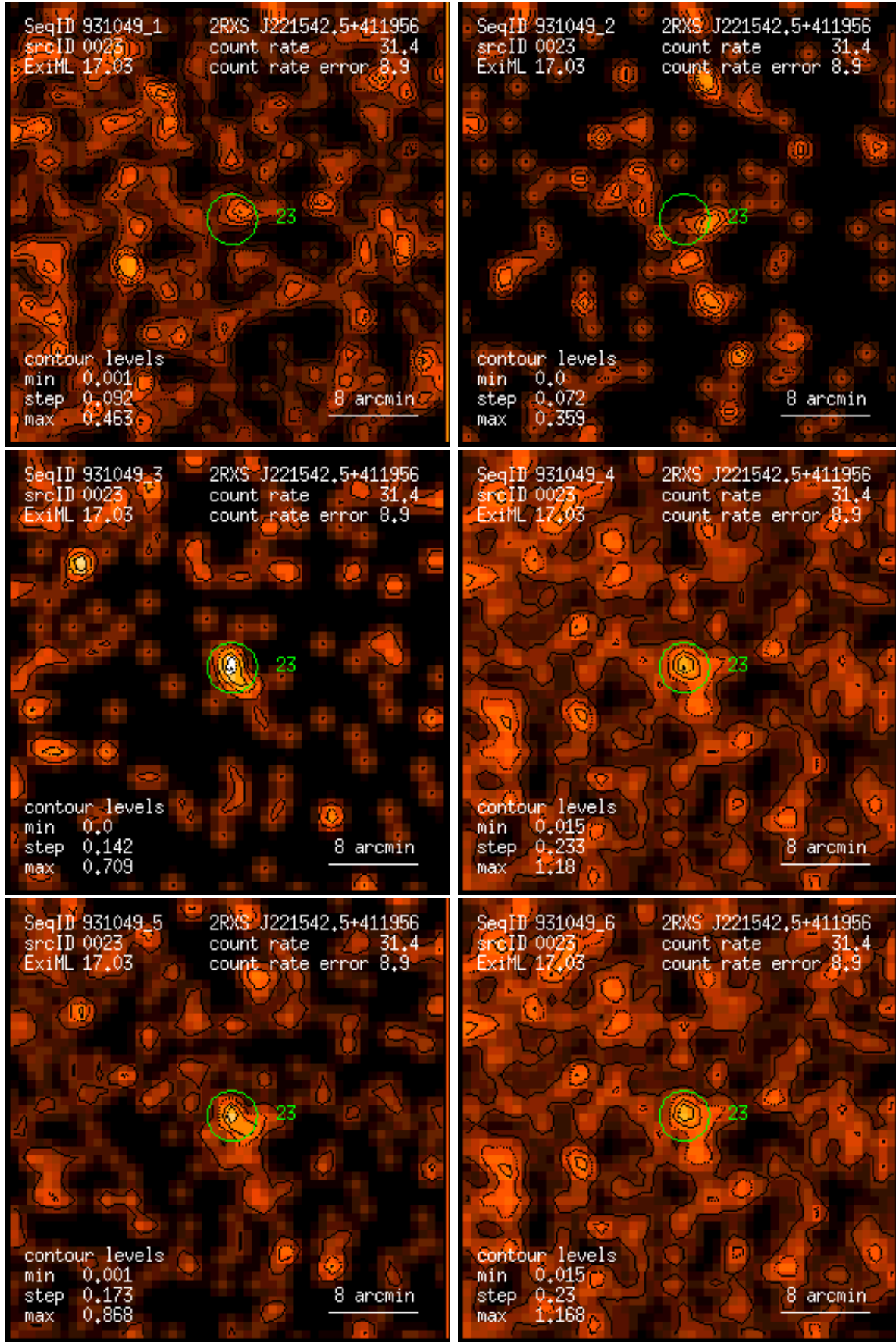
Figure 23: RASS 931049: detection 0023: band rate images, Gaussian filter: (1) PSPC channels 11 – 41, (2) 52 – 90, (3) 91 – 201, (4) 11 – 235, (5) 52 – 201, (6) 11 – 201. Broad band rates in counts/ks. Band rate contour levels in counts/ks/arcmin 2 .
