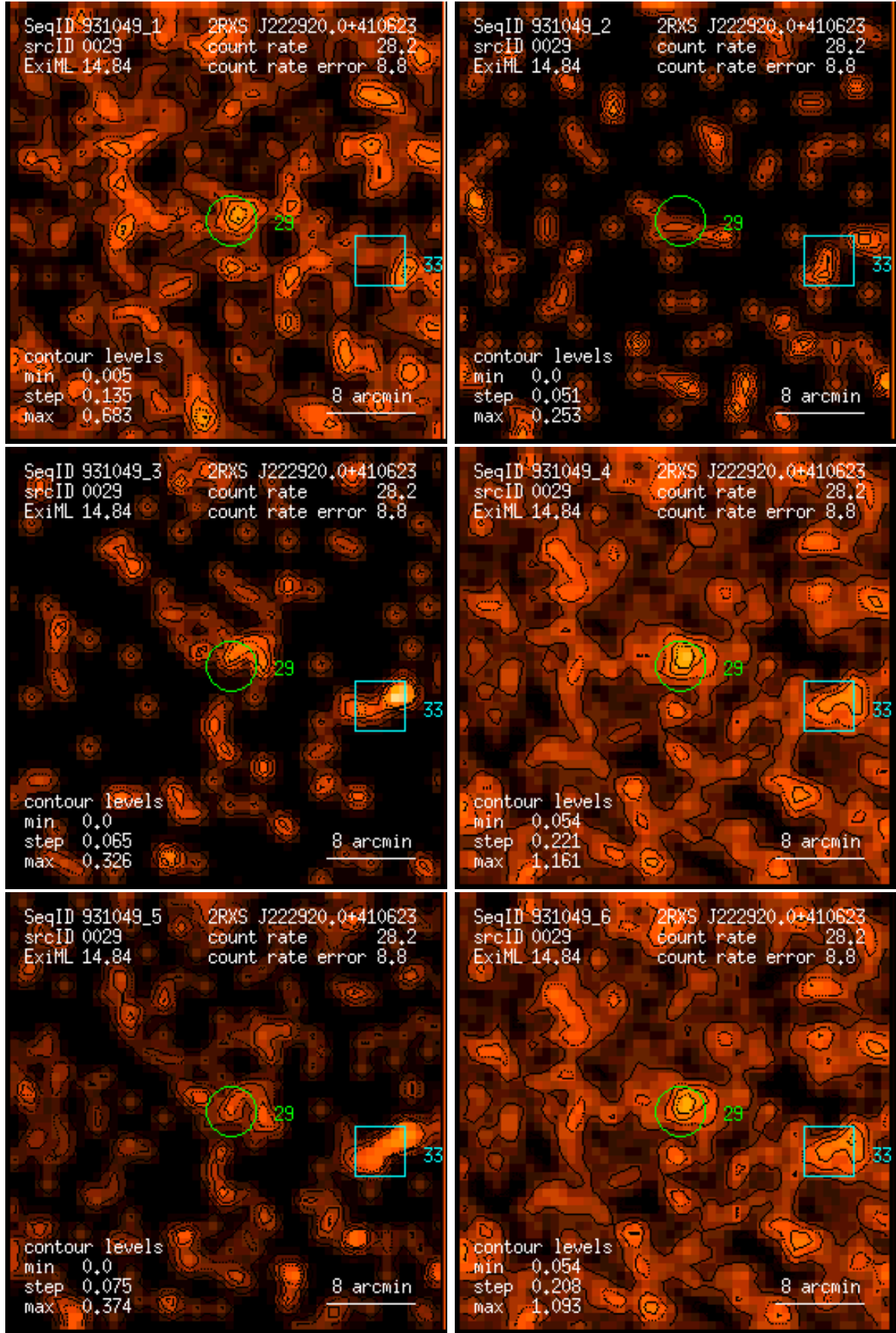
Figure 29: RASS 931049: detection 0029: band rate images, Gaussian filter: (1) PSPC channels 11 – 41, (2) 52 – 90, (3) 91 – 201, (4) 11 – 235, (5) 52 – 201, (6) 11 – 201. Broad band rates in counts/ks. Band rate contour levels in counts/ks/arcmin 2 .
