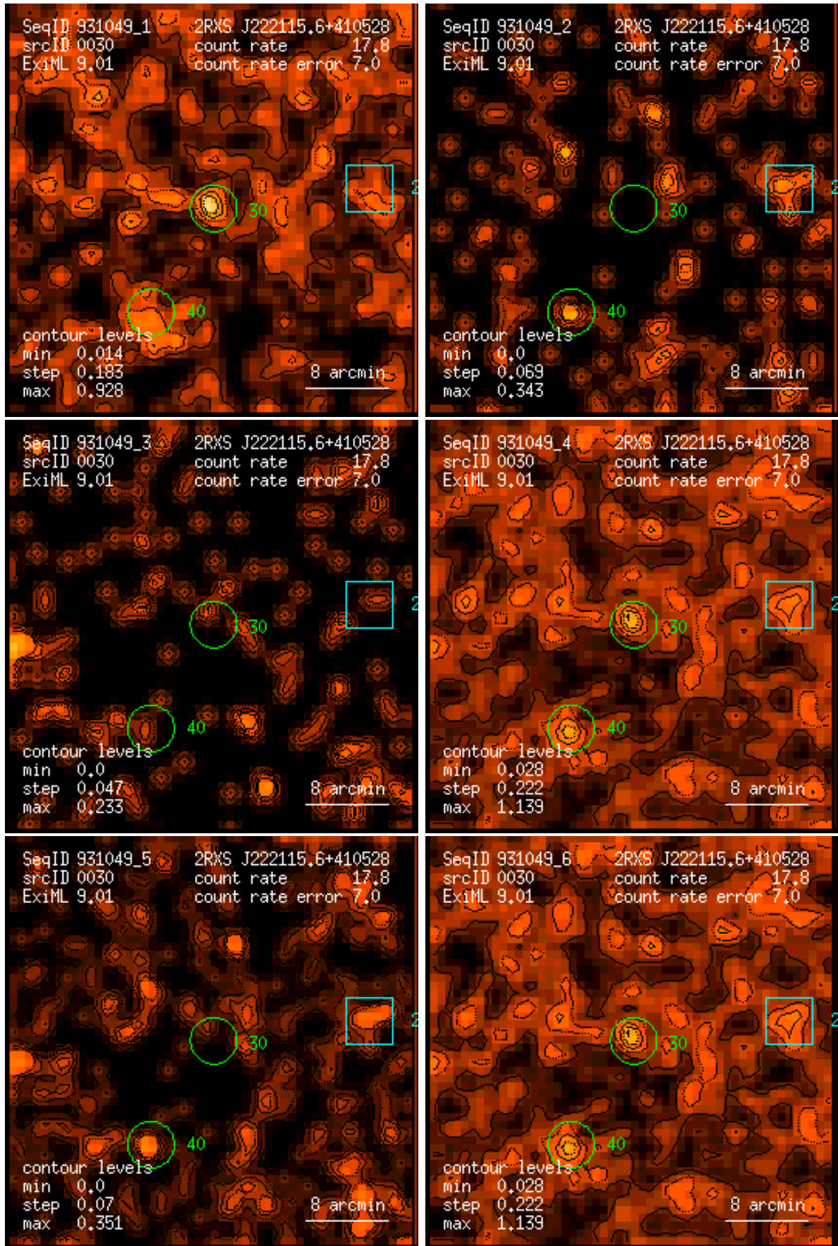
Figure 30: RASS 931049: detection 0030: band rate images, Gaussian filter: (1) PSPC channels 11 – 41, (2) 52 – 90, (3) 91 – 201, (4) 11 – 235, (5) 52 – 201, (6) 11 – 201. Broad band rates in counts/ks. Band rate contour levels in counts/ks/arcmin 2 .
