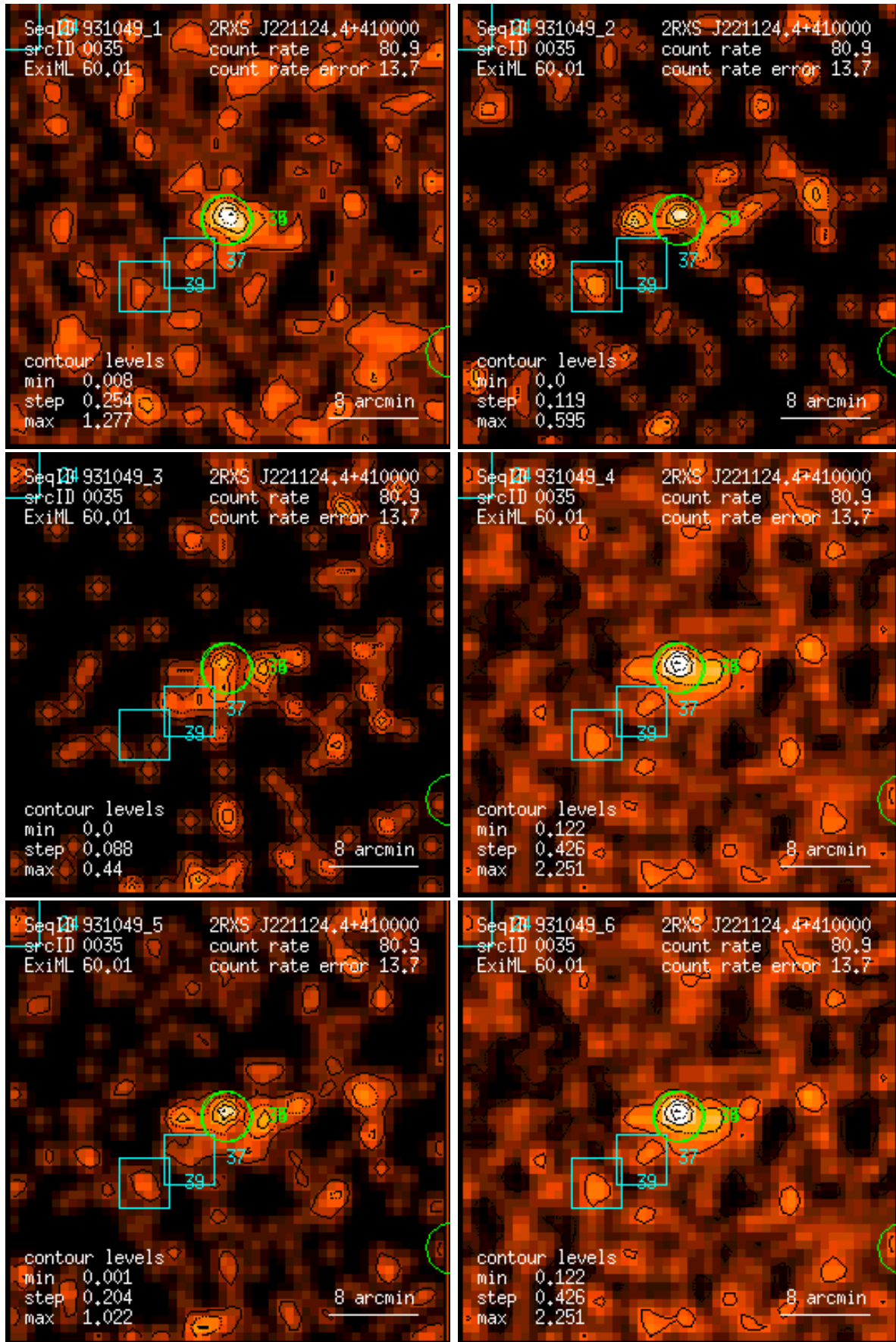
Figure 35: RASS 931049: detection 0035: band rate images, Gaussian filter: (1) PSPC channels 11 – 41, (2) 52 – 90, (3) 91 – 201, (4) 11 – 235, (5) 52 – 201, (6) 11 – 201. Broad band rates in counts/ks. Band rate contour levels in counts/ks/arcmin 2 .
