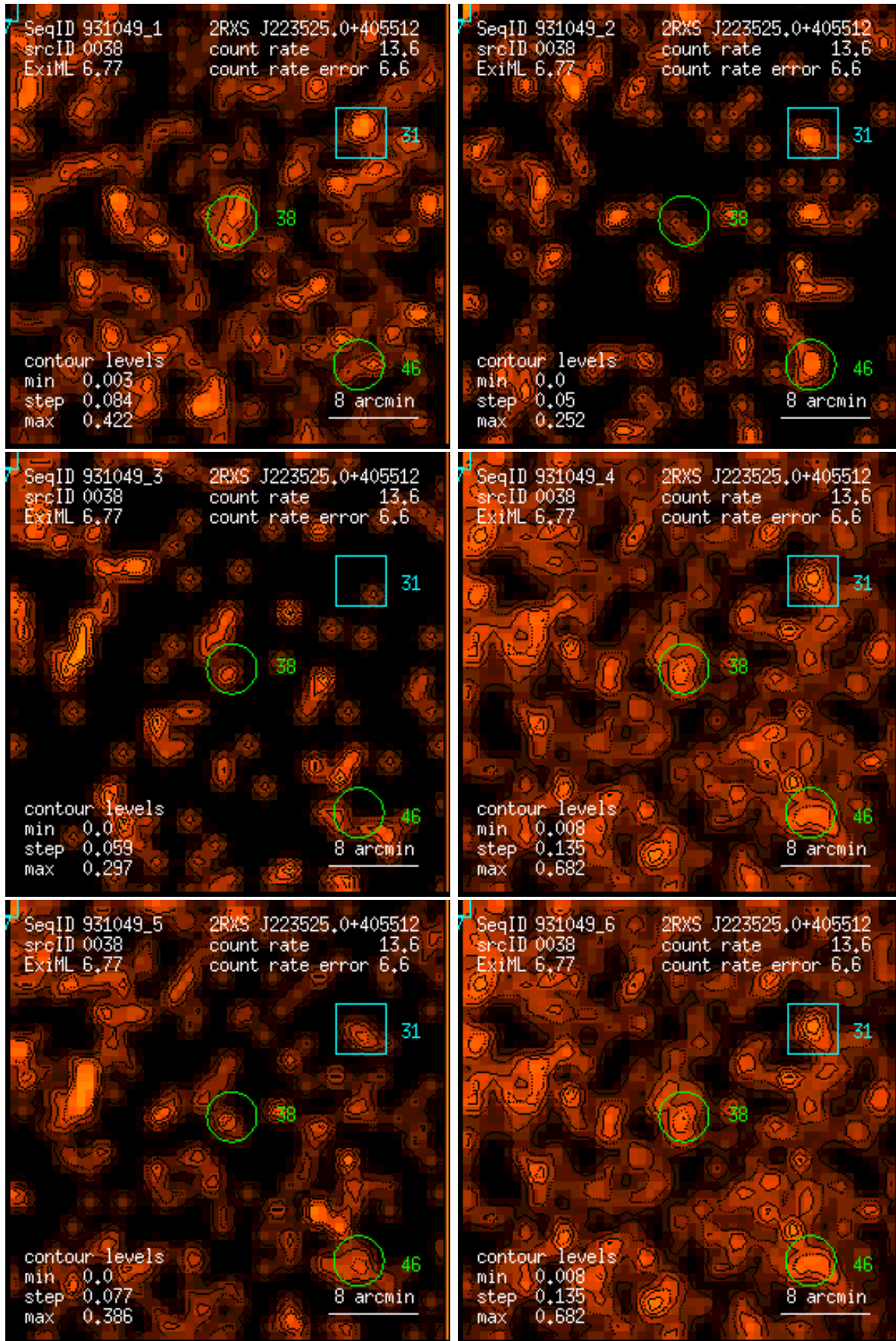
Figure 38: RASS 931049: detection 0038: band rate images, Gaussian filter: (1) PSPC channels 11 – 41, (2) 52 – 90, (3) 91 – 201, (4) 11 – 235, (5) 52 – 201, (6) 11 – 201. Broad band rates in counts/ks. Band rate contour levels in counts/ks/arcmin 2 .
