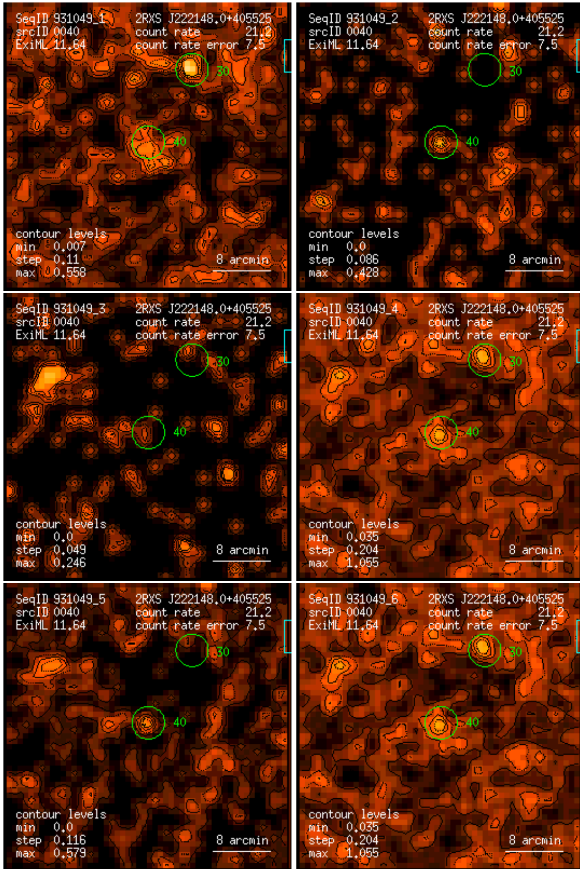
Figure 40: RASS 931049: detection 0040: band rate images, Gaussian filter: (1) PSPC channels 11 – 41, (2) 52 – 90, (3) 91 – 201, (4) 11 – 235, (5) 52 – 201, (6) 11 – 201. Broad band rates in counts/ks. Band rate contour levels in counts/ks/arcmin 2 .
