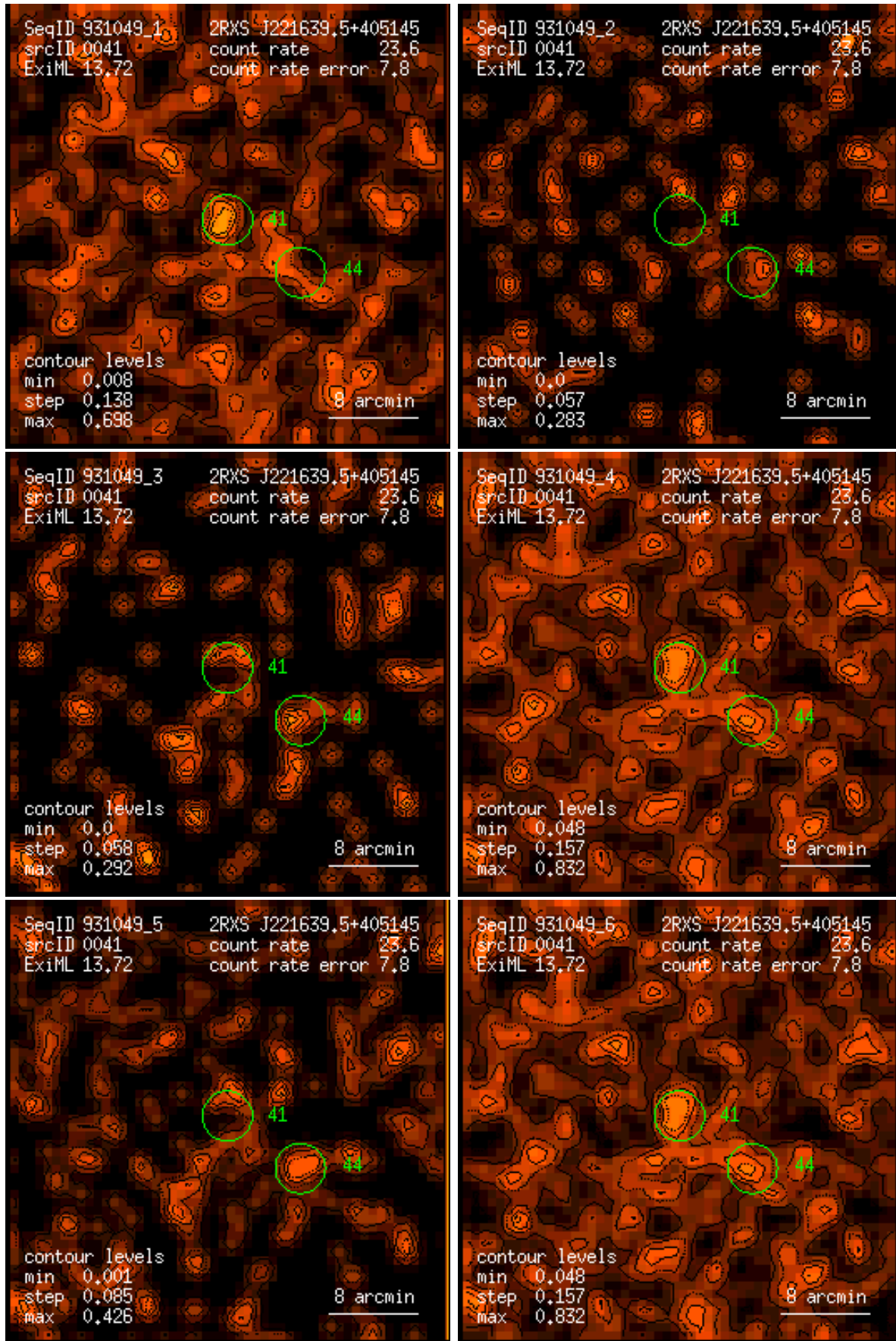
Figure 41: RASS 931049: detection 0041: band rate images, Gaussian filter: (1) PSPC channels 11 – 41, (2) 52 – 90, (3) 91 – 201, (4) 11 – 235, (5) 52 – 201, (6) 11 – 201. Broad band rates in counts/ks. Band rate contour levels in counts/ks/arcmin 2 .
