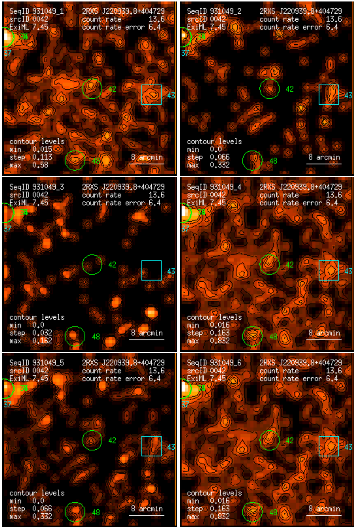
Figure 42: RASS 931049: detection 0042: band rate images, Gaussian filter: (1) PSPC channels 11 – 41, (2) 52 – 90, (3) 91 – 201, (4) 11 – 235, (5) 52 – 201, (6) 11 – 201. Broad band rates in counts/ks. Band rate contour levels in counts/ks/arcmin 2 .
