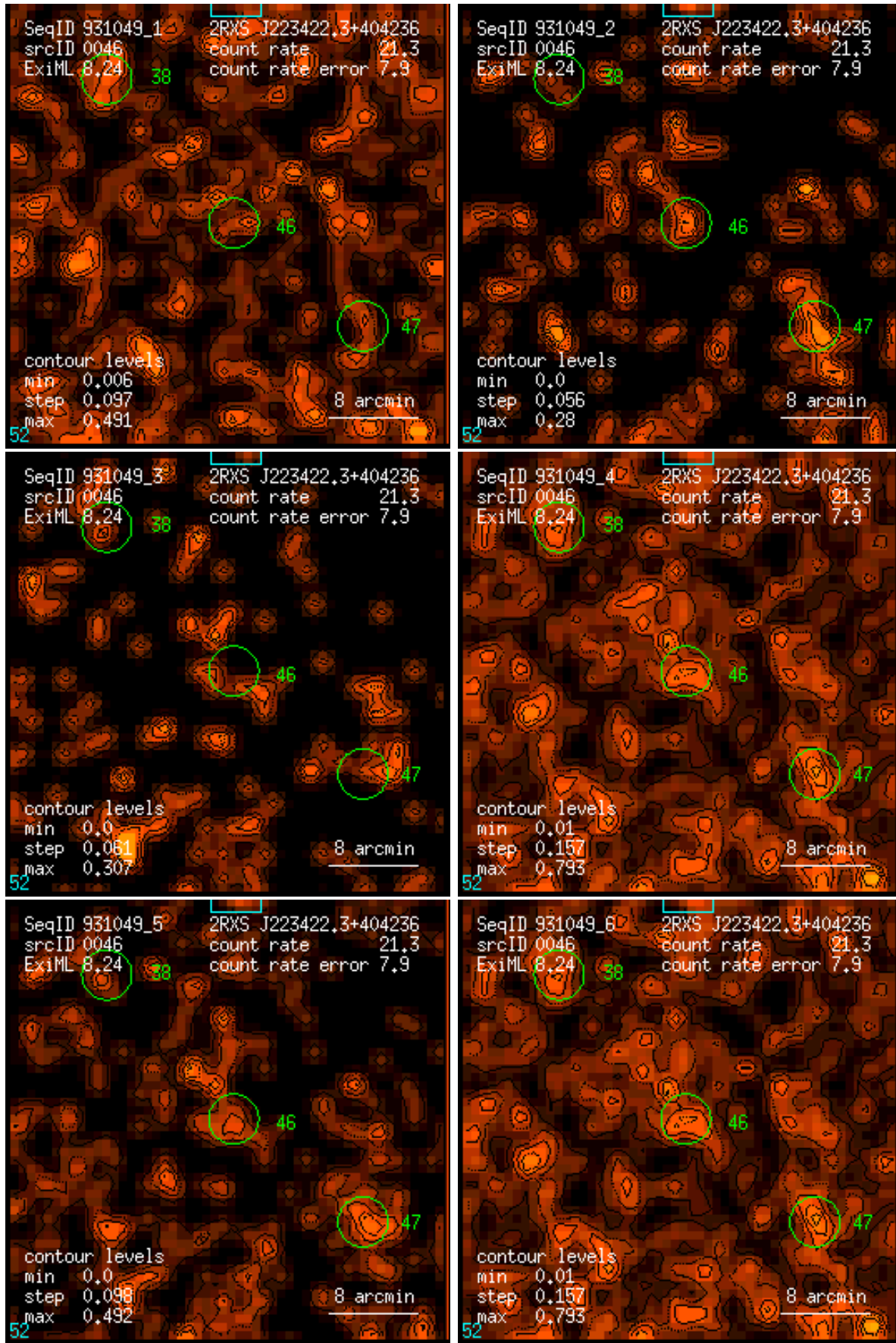
Figure 46: RASS 931049: detection 0046: band rate images, Gaussian filter: (1) PSPC channels 11 – 41, (2) 52 – 90, (3) 91 – 201, (4) 11 – 235, (5) 52 – 201, (6) 11 – 201. Broad band rates in counts/ks. Band rate contour levels in counts/ks/arcmin 2 .
