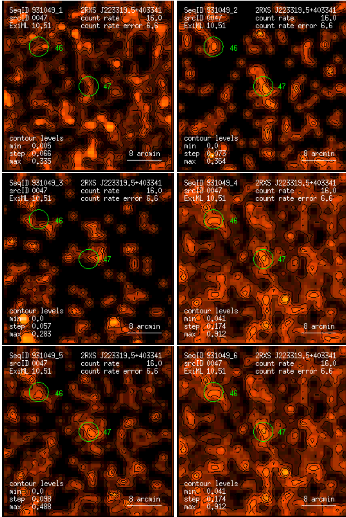
Figure 47: RASS 931049: detection 0047: band rate images, Gaussian filter: (1) PSPC channels 11 – 41, (2) 52 – 90, (3) 91 – 201, (4) 11 – 235, (5) 52 – 201, (6) 11 – 201. Broad band rates in counts/ks. Band rate contour levels in counts/ks/arcmin 2 .
