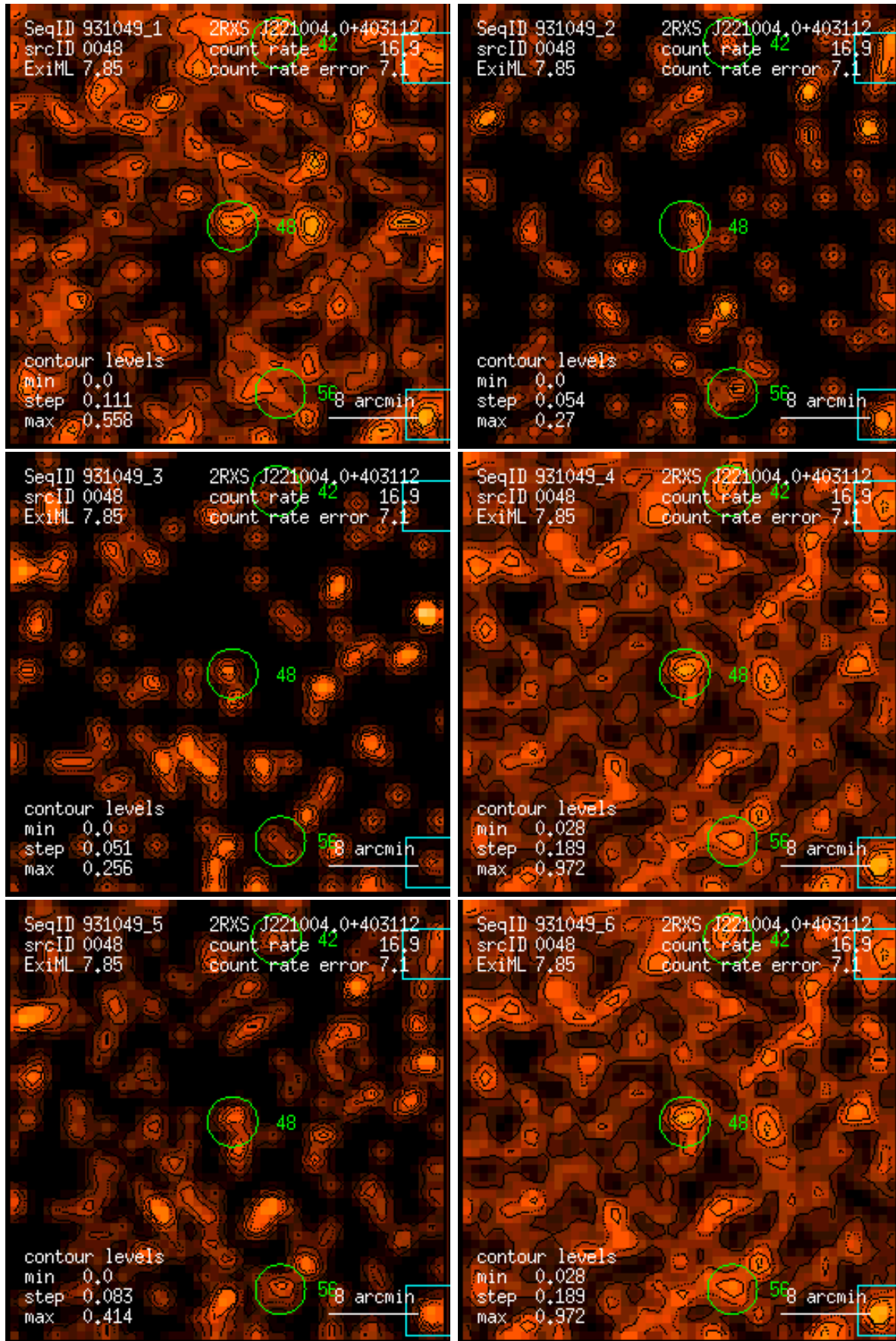
Figure 48: RASS 931049: detection 0048: band rate images, Gaussian filter: (1) PSPC channels 11 – 41, (2) 52 – 90, (3) 91 – 201, (4) 11 – 235, (5) 52 – 201, (6) 11 – 201. Broad band rates in counts/ks. Band rate contour levels in counts/ks/arcmin 2 .
