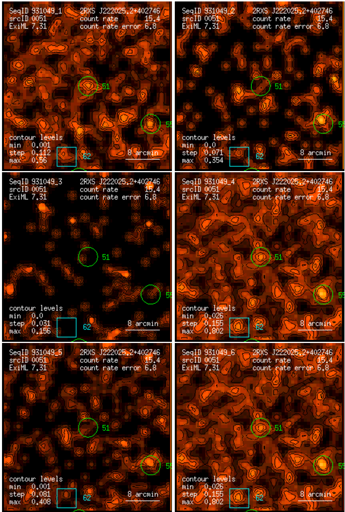
Figure 51: RASS 931049: detection 0051: band rate images, Gaussian filter: (1) PSPC channels 11 – 41, (2) 52 – 90, (3) 91 – 201, (4) 11 – 235, (5) 52 – 201, (6) 11 – 201. Broad band rates in counts/ks. Band rate contour levels in counts/ks/arcmin 2 .
