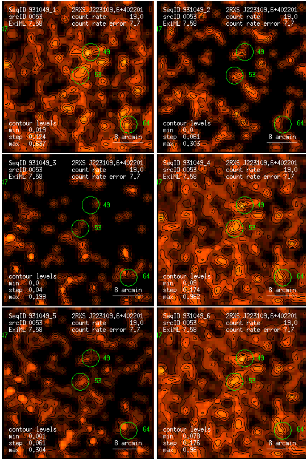
Figure 53: RASS 931049: detection 0053: band rate images, Gaussian filter: (1) PSPC channels 11 – 41, (2) 52 – 90, (3) 91 – 201, (4) 11 – 235, (5) 52 – 201, (6) 11 – 201. Broad band rates in counts/ks. Band rate contour levels in counts/ks/arcmin 2 .
