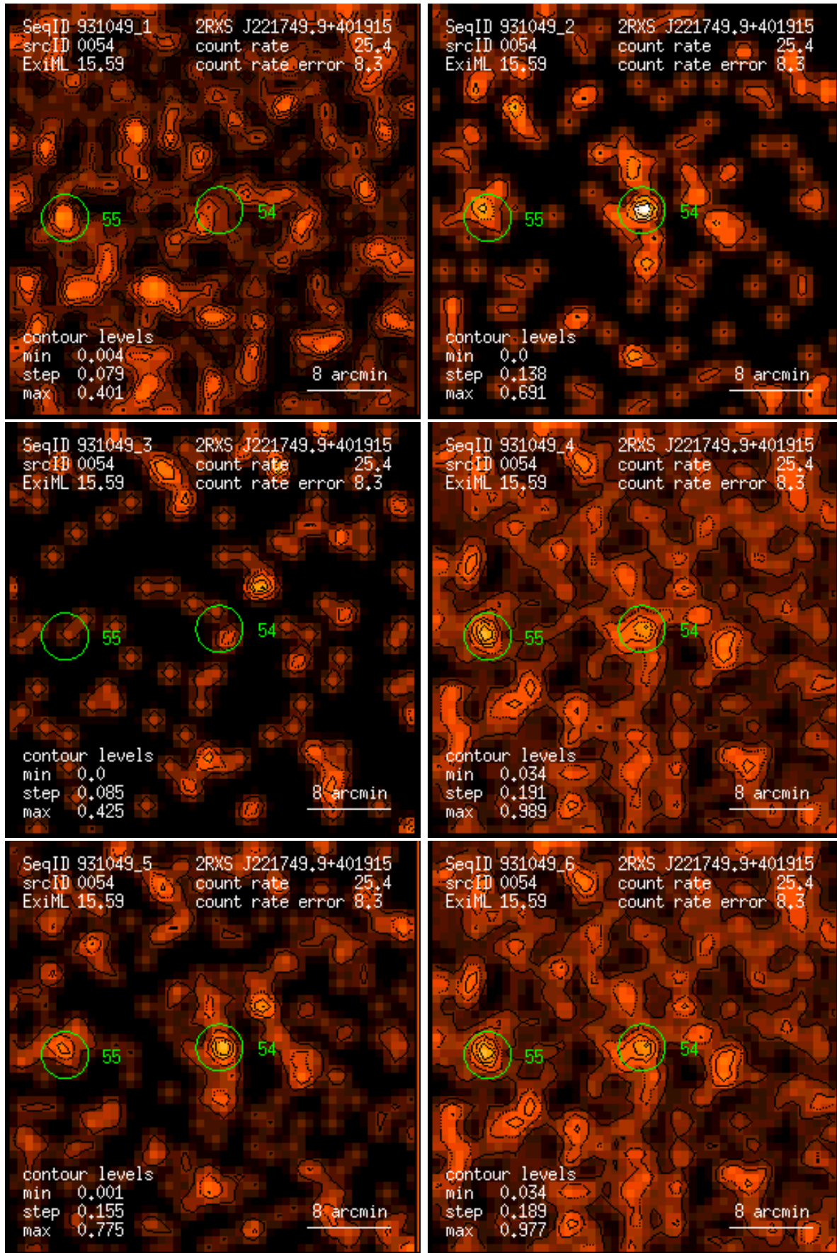
Figure 54: RASS 931049: detection 0054: band rate images, Gaussian filter: (1) PSPC channels 11 – 41, (2) 52 – 90, (3) 91 – 201, (4) 11 – 235, (5) 52 – 201, (6) 11 – 201. Broad band rates in counts/ks. Band rate contour levels in counts/ks/arcmin 2 .
